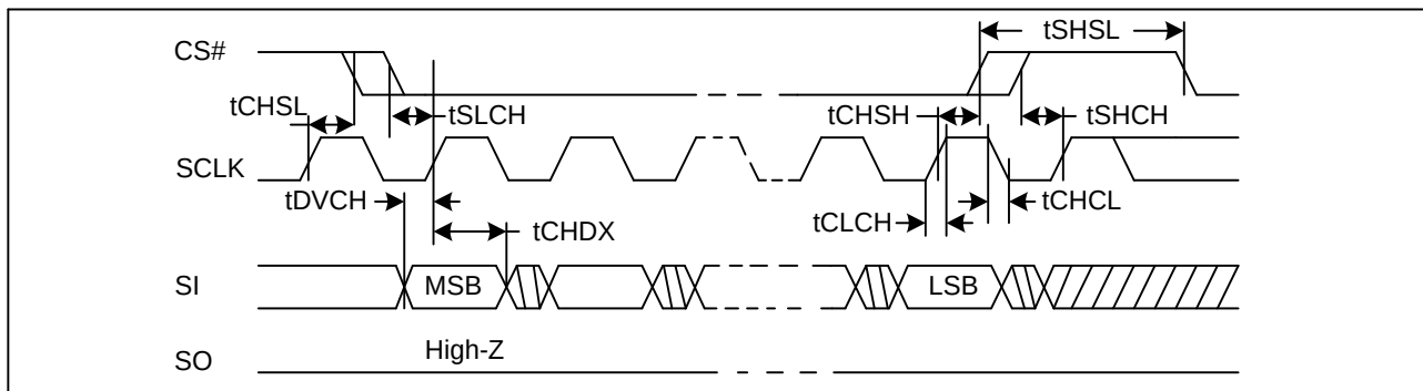
Figure 63. Input Timing
