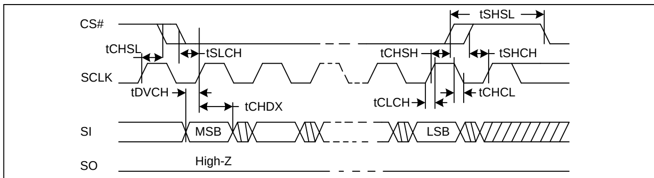
Figure 38. Input Timing
