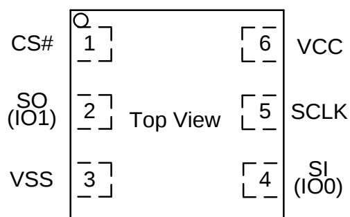
6 - LEAD USON
