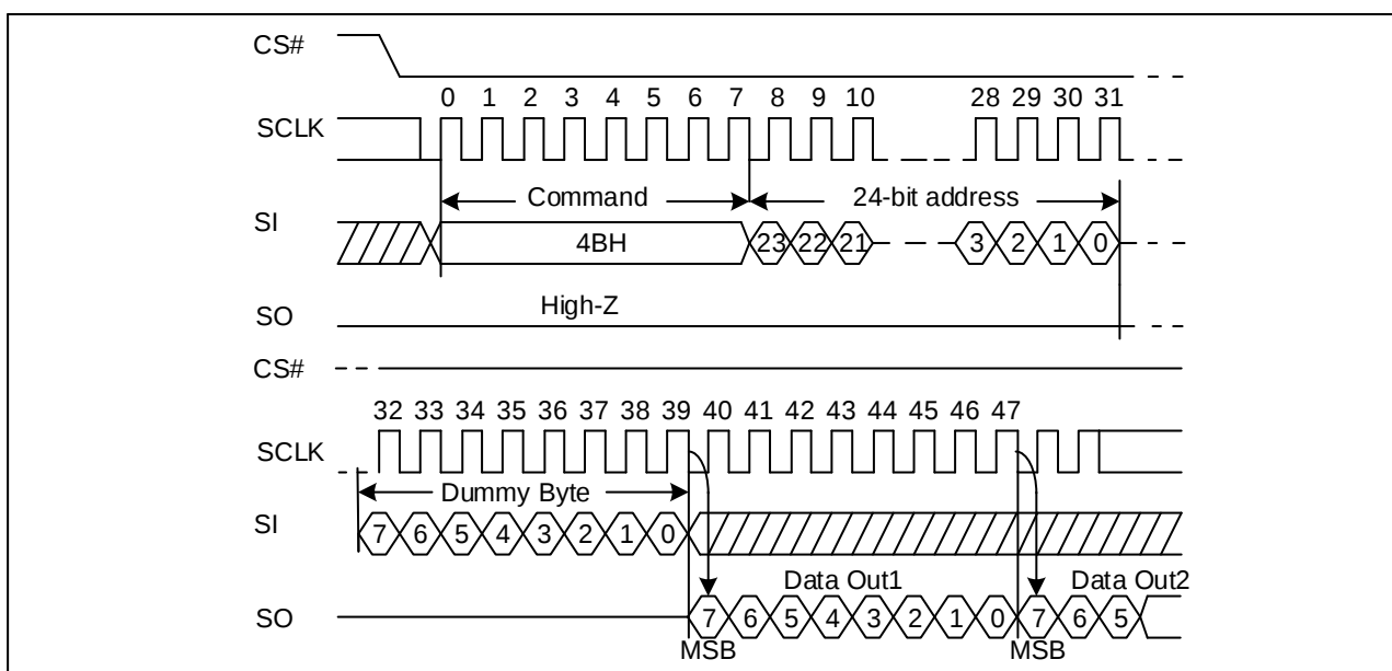
Figure18. Read Unique ID Sequence Diagram
