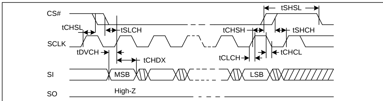
Figure 25. Input Timing
