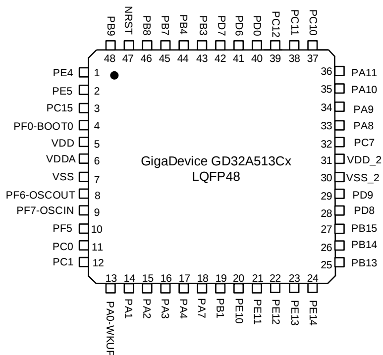
Figure 2-4. GD32A513Cx LQFP48 pinouts
