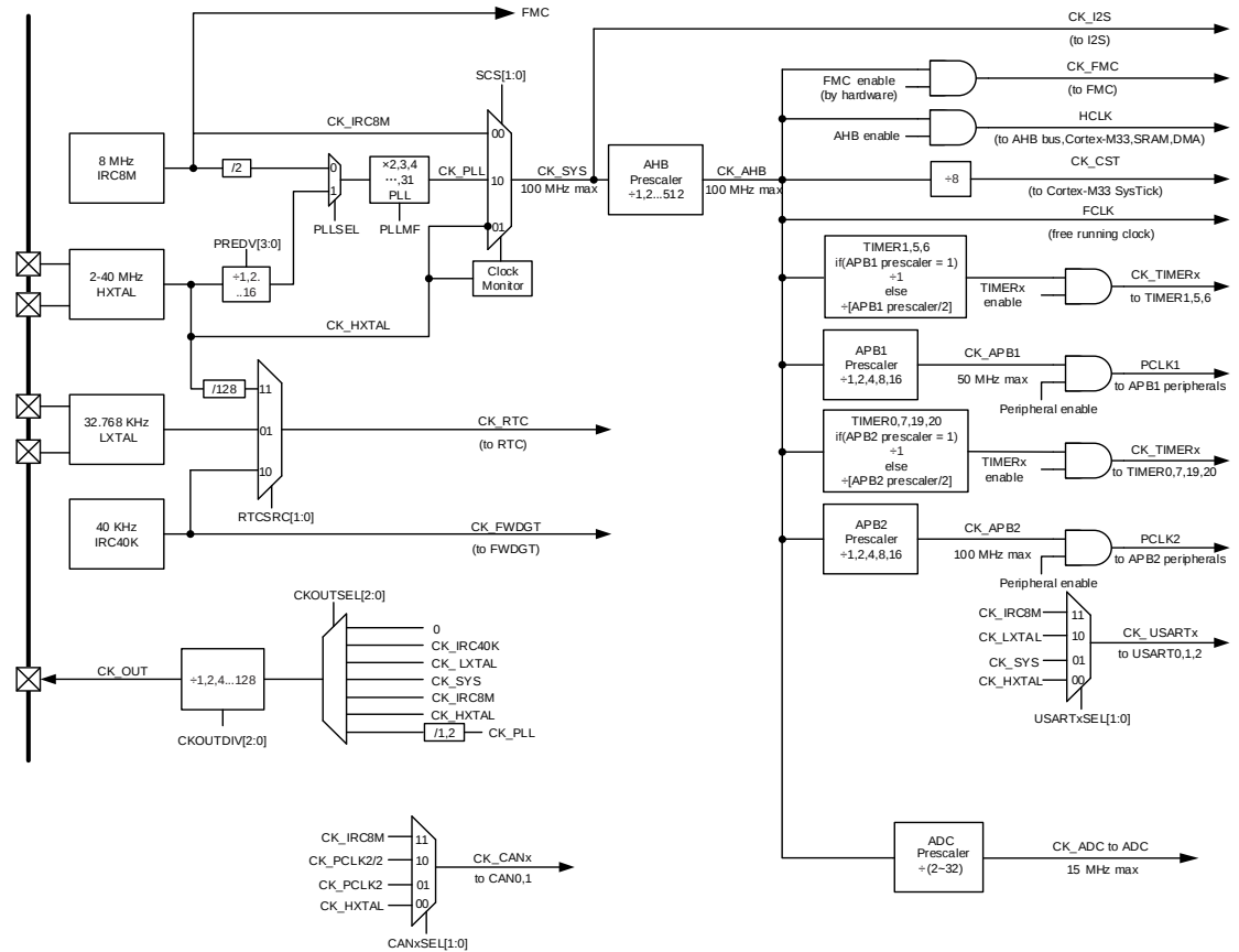
Figure 2-6. GD32A513xx clock tree
