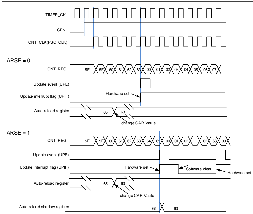
Figure 16-71. Timing chart of up counting, change TIMERx_CAR ongoing
