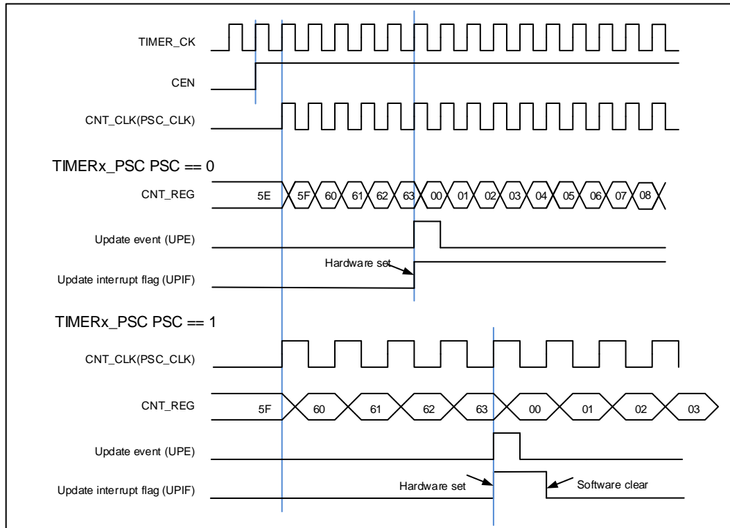
Figure 16-37. Timing chart of up counting mode, PSC=0/1
