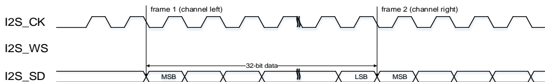
Figure 19-17. I2S Phillips standard timing diagram (DTLEN=10, CHLEN=1, CKPL=0)
