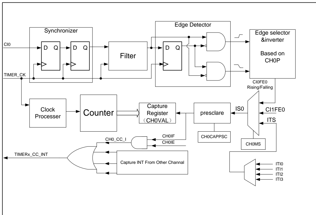
Figure 16-42. Input capture logic
