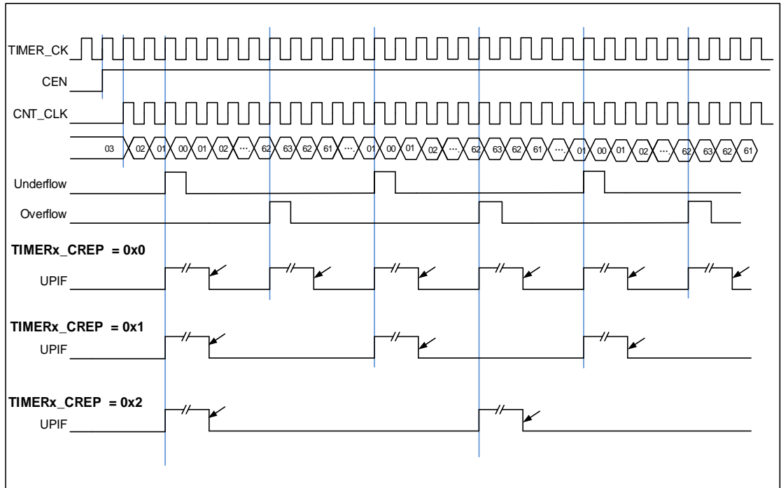
Figure 16-9. Repetition counter timing chart of center-aligned counting mode
