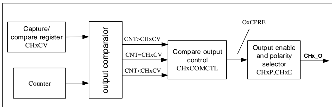
Figure 16-59. Output compare logic (x=0,1)
