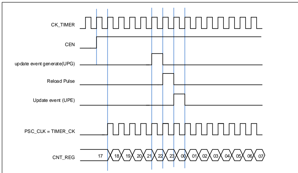
Figure 16-35. Normal mode, internal clock divided by 1
