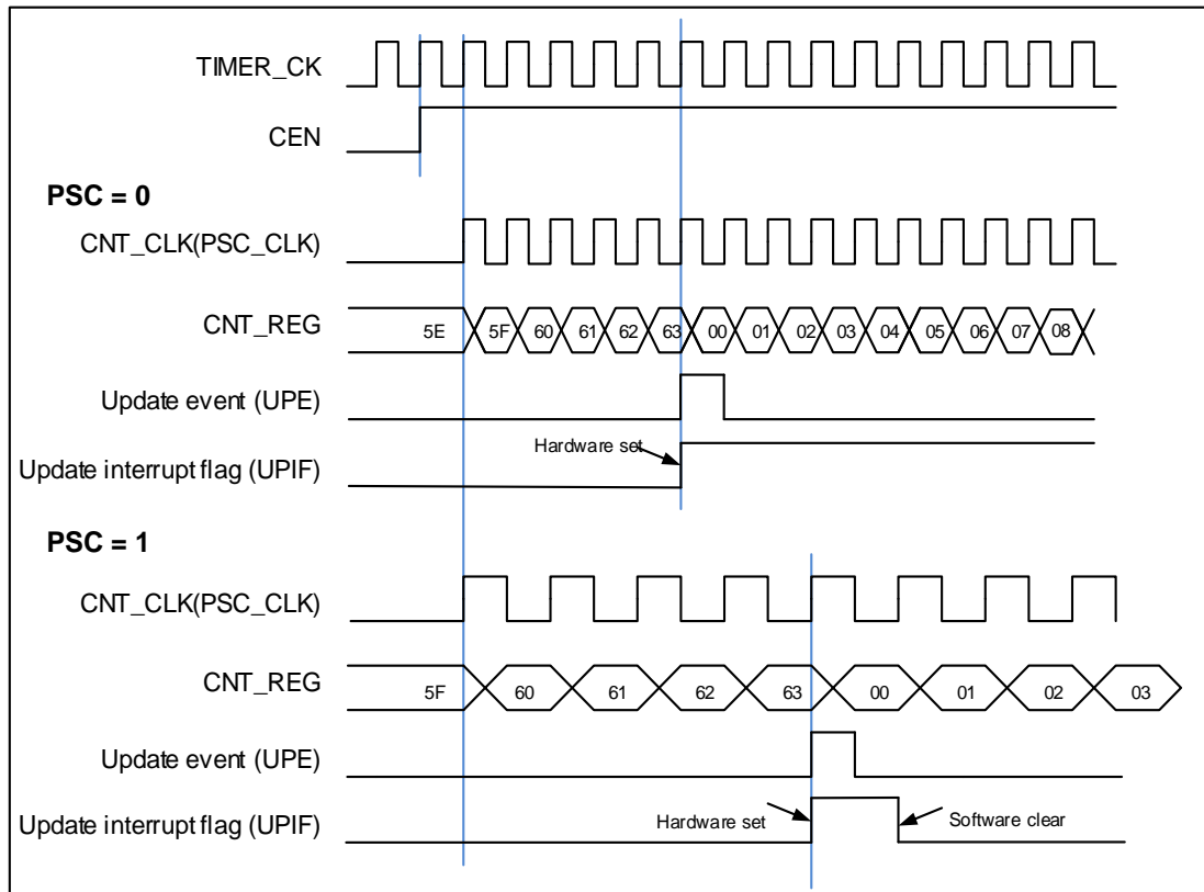
Figure 16-4. Timing chart of up counting mode, PSC=0/1
