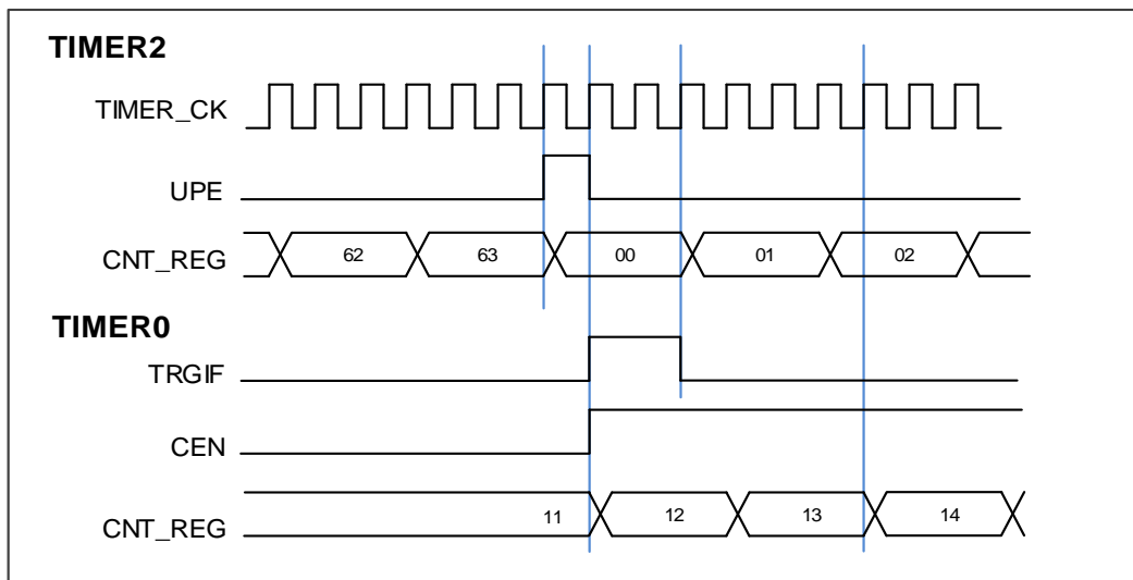
Figure 16-30. Trigger mode of TIMER0 controlled by update signal of TIMER2
