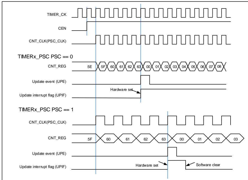
Figure 16-78. Timing chart of up counting mode, PSC=0/1
