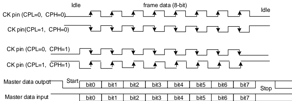
Figure 17-12. 8-bit format USART synchronous waveform (CLEN=1)
