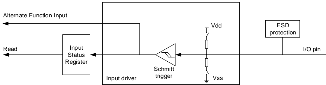
Figure 8-2. Input configuration
