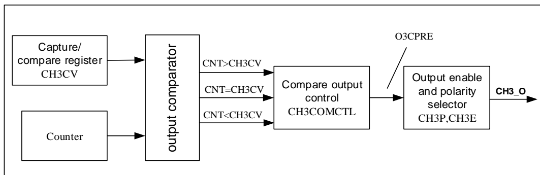
Figure 16-14. Output compare logic (CH3_O)
