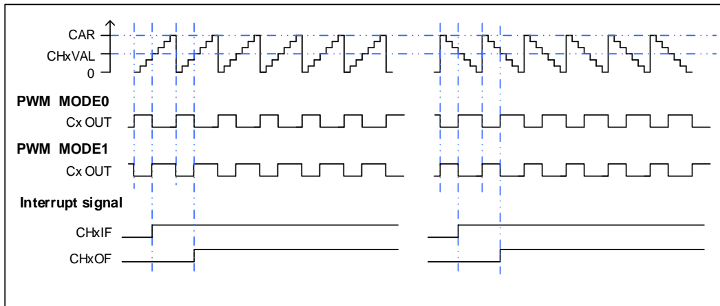
Figure 16-16. Timing chart of EAPWM
