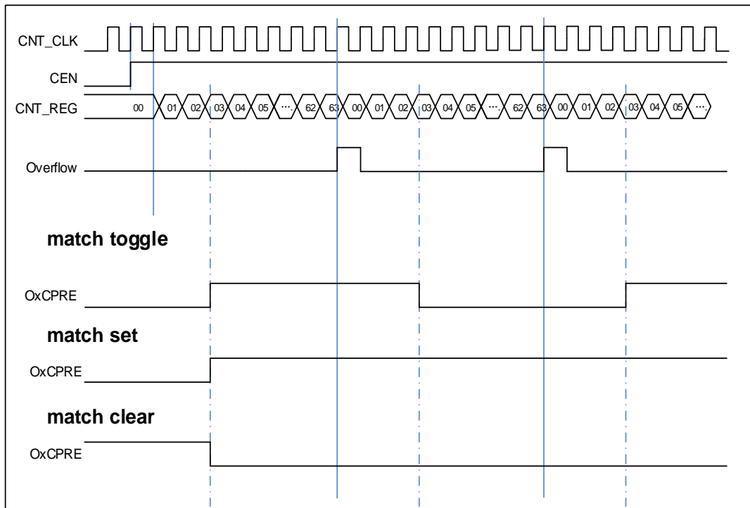
Figure 16-15. Output-compare in three modes
