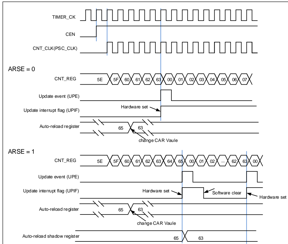
Figure 16-79. Timing chart of up counting mode, change TIMERx_CAR ongoing
