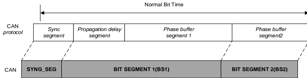
Figure 21-11. The bit time
