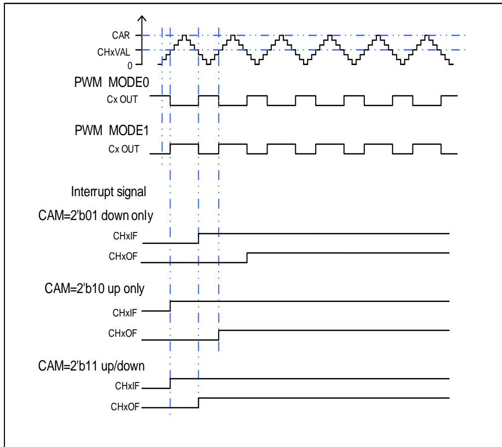
Figure 16-46. Timing chart of CAPWM
