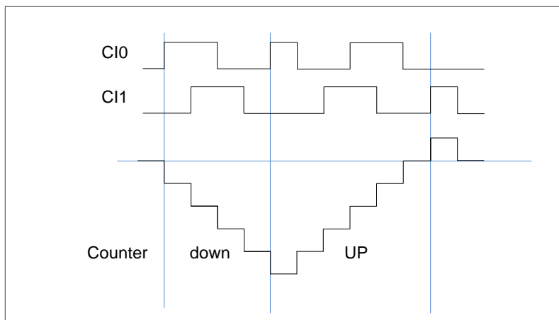
Figure 16-21. Example of encoder interface mode with CI0FE0 polarity inverted
