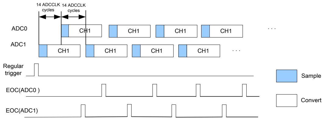
Figure 12-17. Follow-up slow mode on 1 channel
