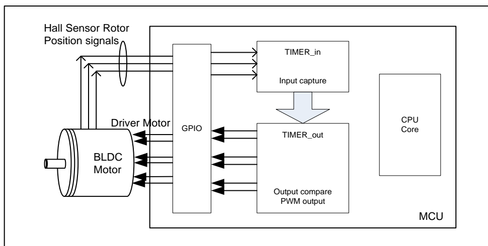
Figure 16-22. Hall sensor is used for BLDC motor
