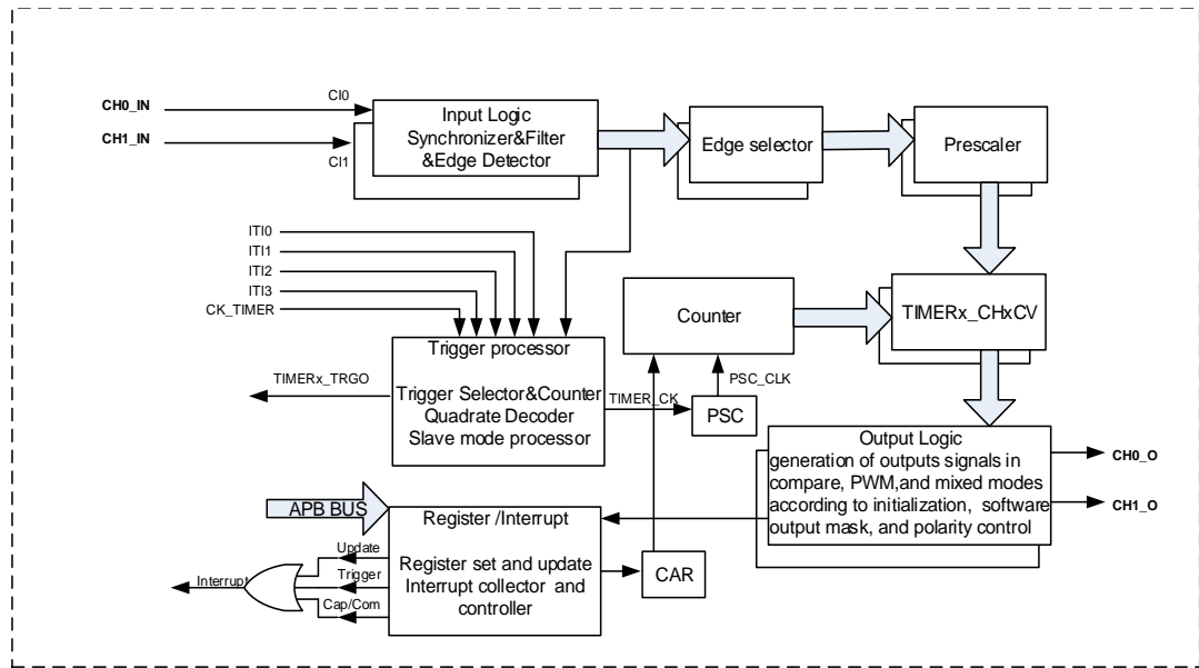
Figure 16-53. General level1 timer block diagram
