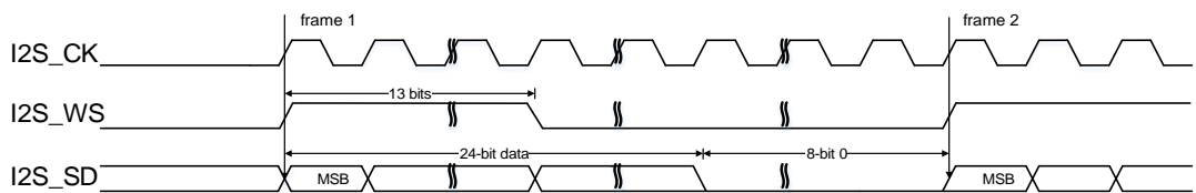
Figure 19-47. PCM standard long frame synchronization mode timing diagram (DTLEN=01, CHLEN=1, CKPL=0)
