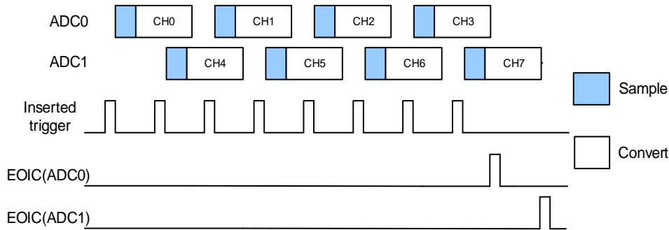
Figure 12-19. Trigger rotation: inserted channels in discontinuous mode
