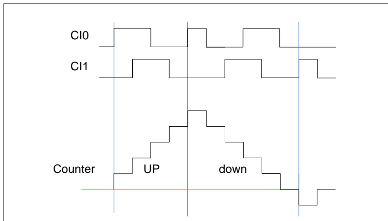
Figure 16-47. Example of counter operation in encoder interface mode
