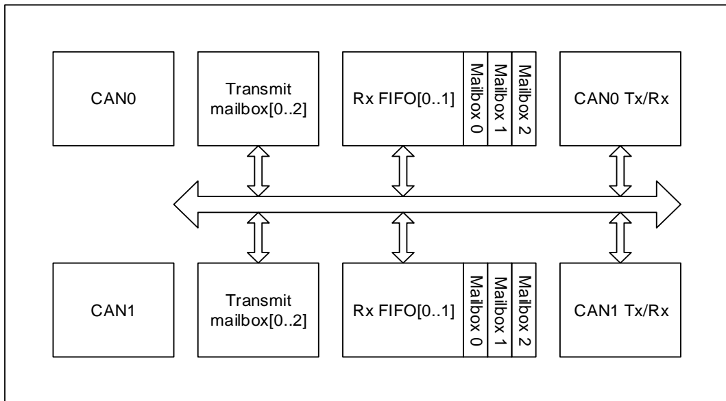
Figure 21-1. CAN module block diagram
