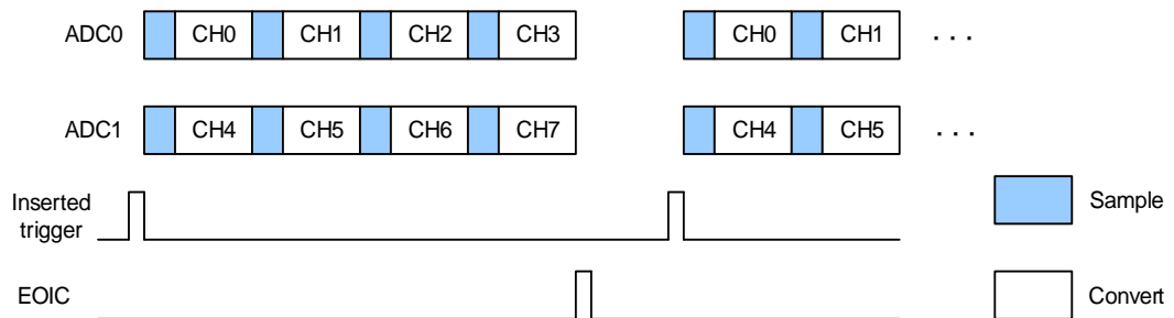
Figure 12-15. Inserted parallel mode on 4 channels
