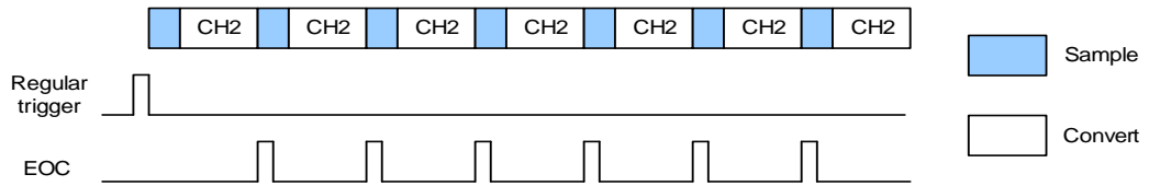
Figure 12-3. Continuous conversion mode
