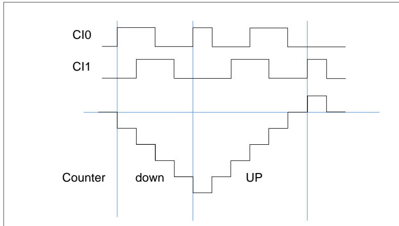
Figure 16-48. Example of encoder interface mode with CI0FE0 polarity inverted
