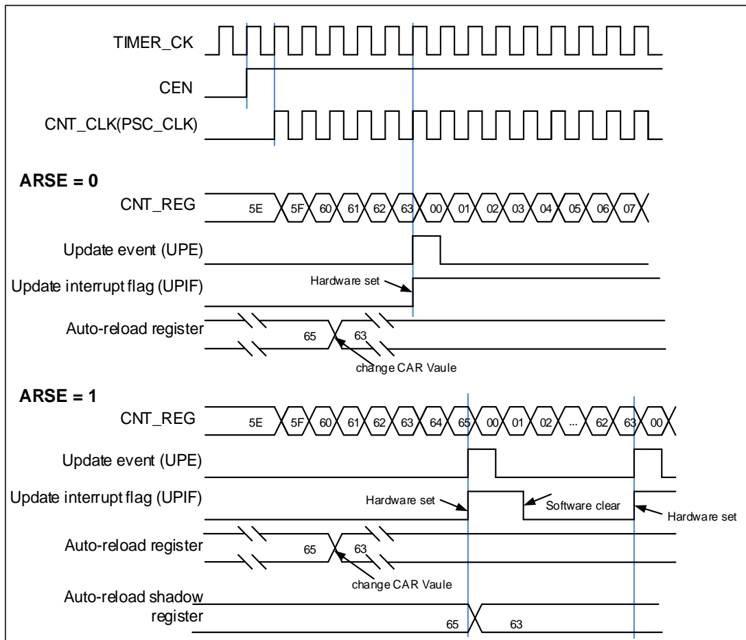
Figure 16-5. Timing chart of up counting mode, change TIMERx_CAR ongoing
