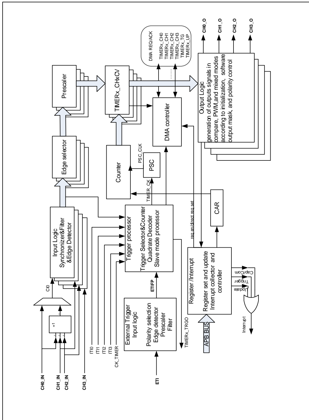
Figure 16-34. General Level 0 timer block diagram
