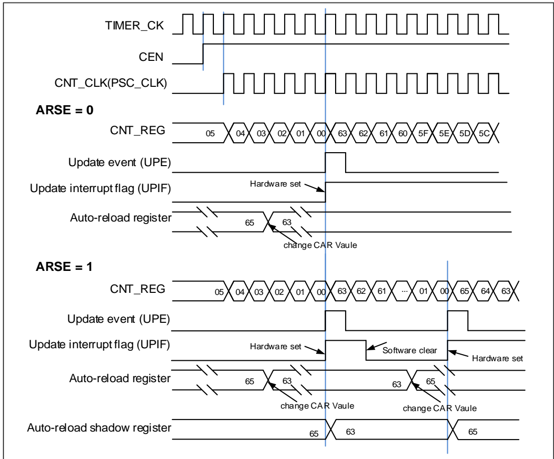
Figure 16-7. Timing chart of down counting mode, change TIMERx_CAR ongoing
