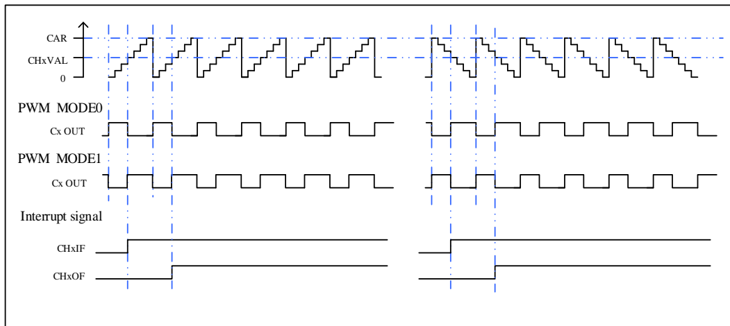
Figure 16-61. Timing chart of EAPWM
