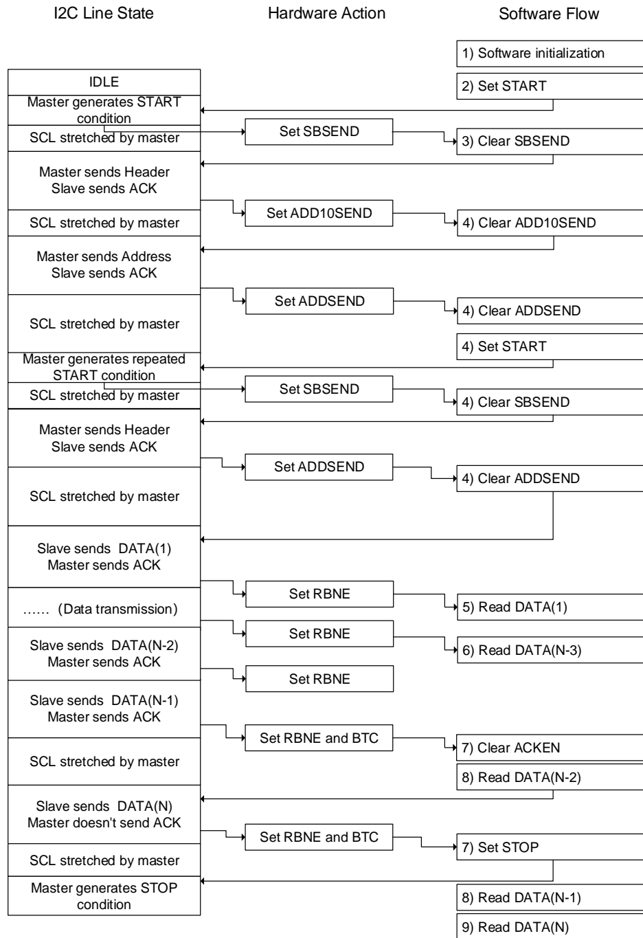
Figure 18-13. Programming model for master receiving mode using solution B
