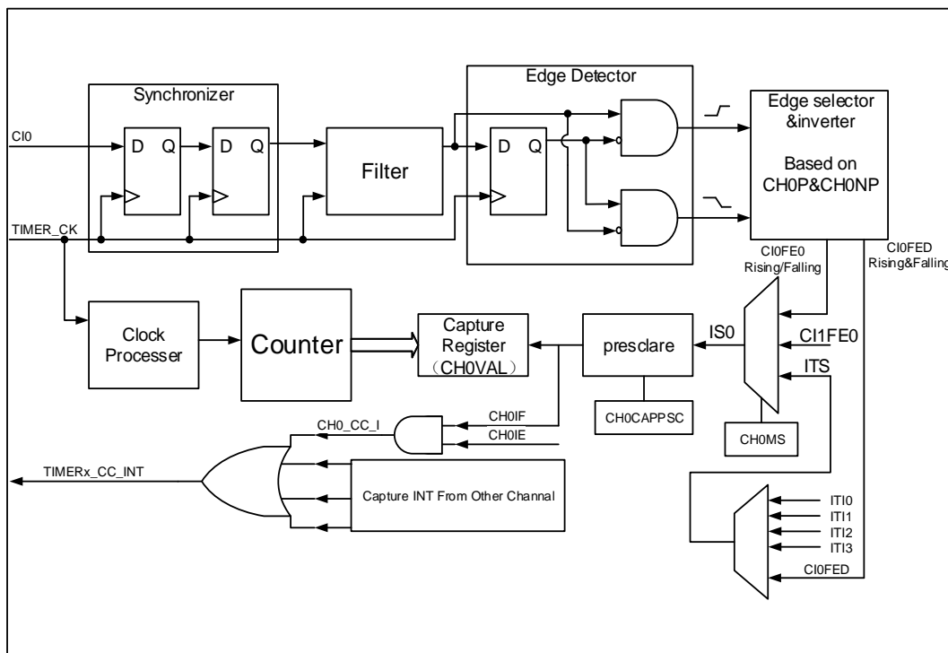
Figure 16-58. Input capture logic
