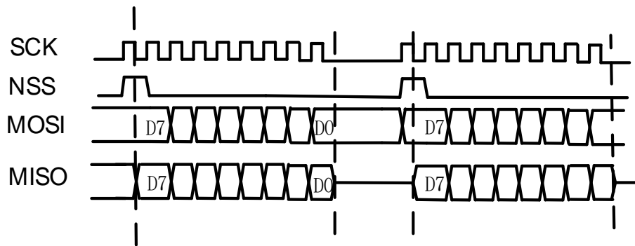
Figure 19-8. Timing diagram of TI master mode with discontinuous transfer
