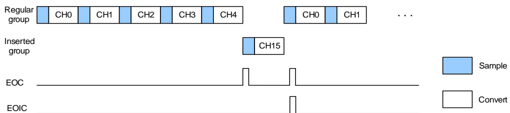
Figure 12-7. Auto-insertion, CNT = 1
