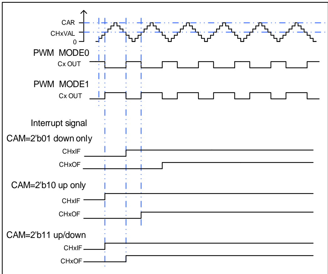
Figure 16-17. Timing chart of CAPWM
