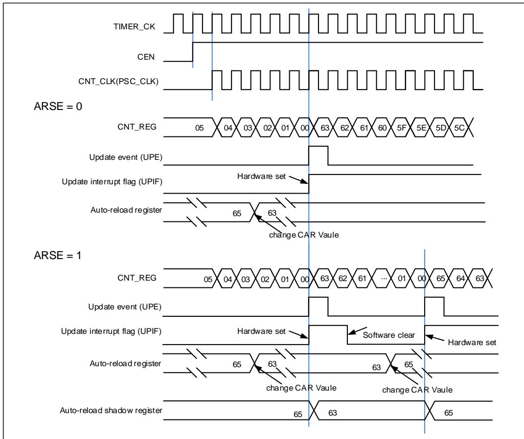
Figure 16-40. Timing chart of down counting mode, change TIMERx_CAR ongoing
