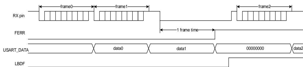
Figure 17-9. Break frame occurs during idle state
