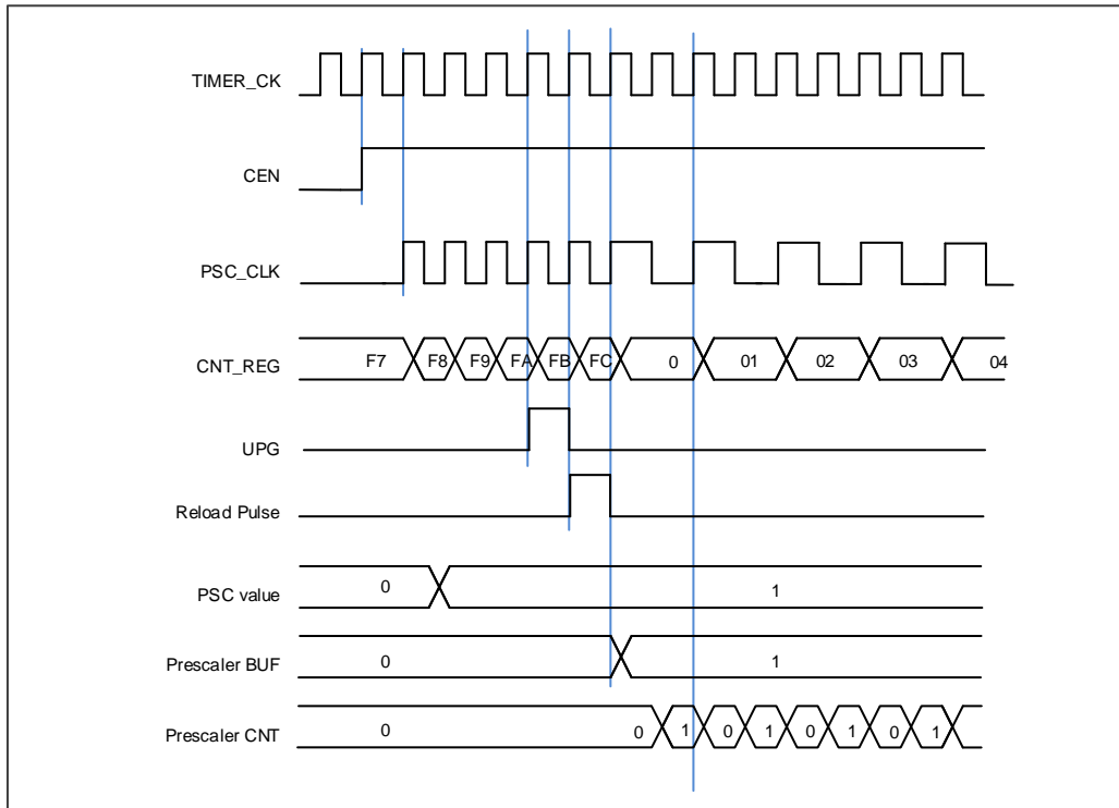
Figure 16-55. Counter timing diagram with prescaler division change from 1 to 2
