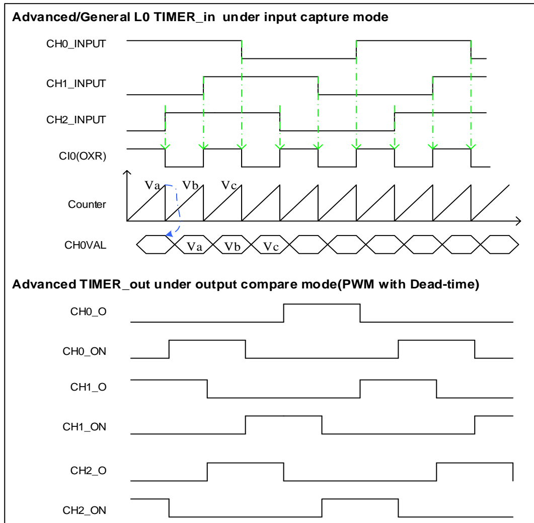
Figure 16-23. Hall sensor timing between two timers
