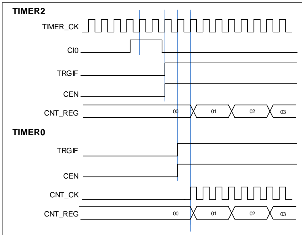
Figure 16-33. Trigger TIMER0 and TIMER2 by the CI0 signal of TIMER2
