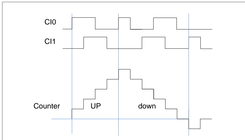
Figure 16-20. Example of counter operation in encoder interface mode
