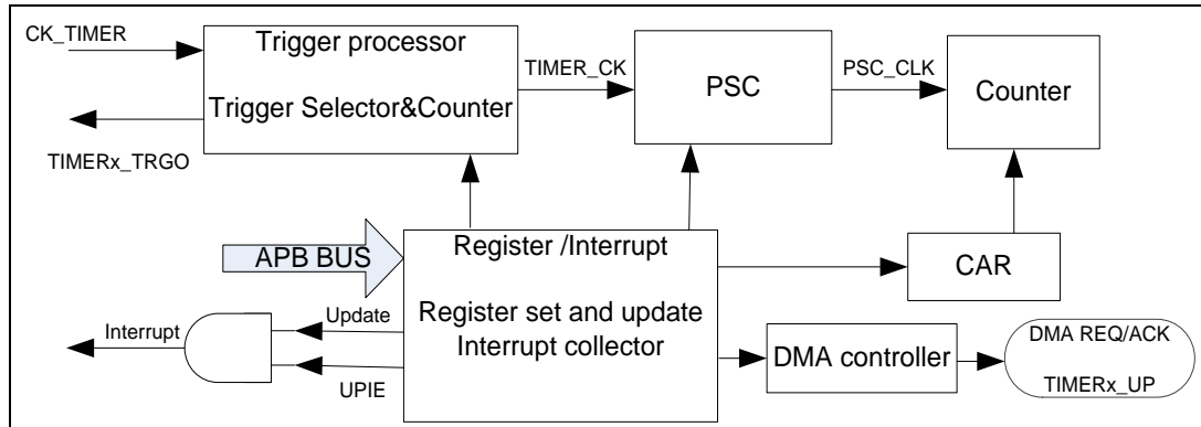
Figure 16-75. Basic timer block diagram
