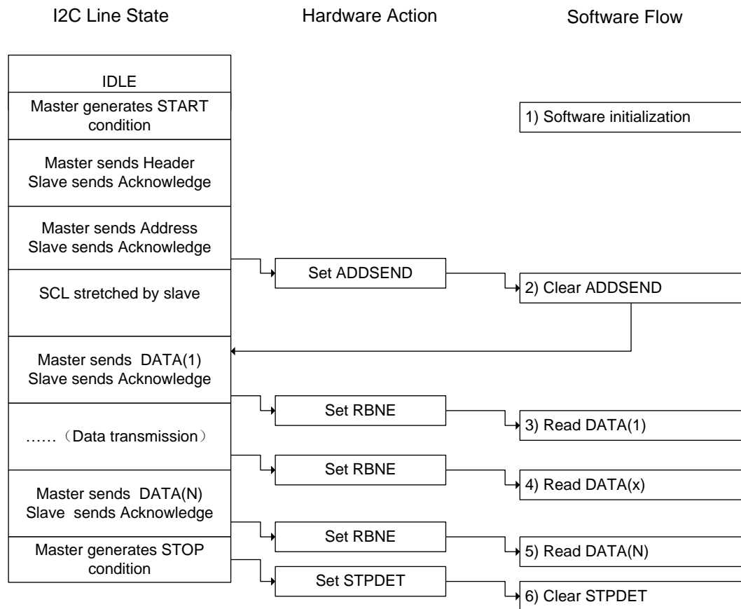
Figure 18-10. Programming model for slave receiving mode
