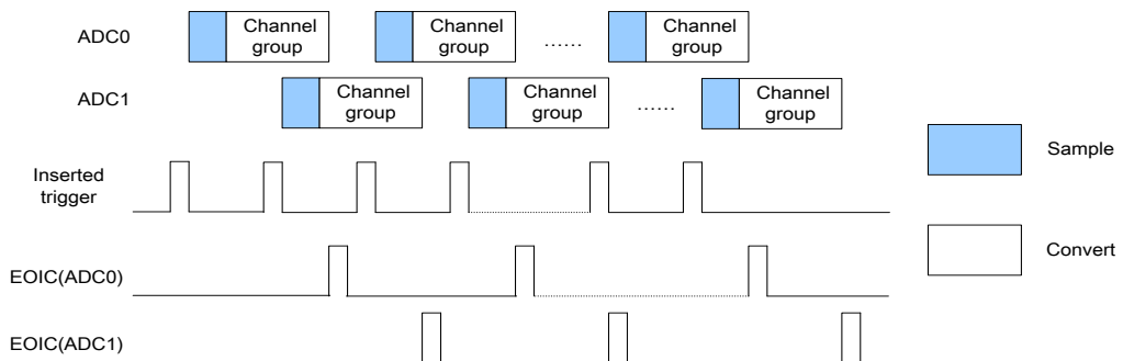
Figure 12-18. Trigger rotation: inserted channel group
