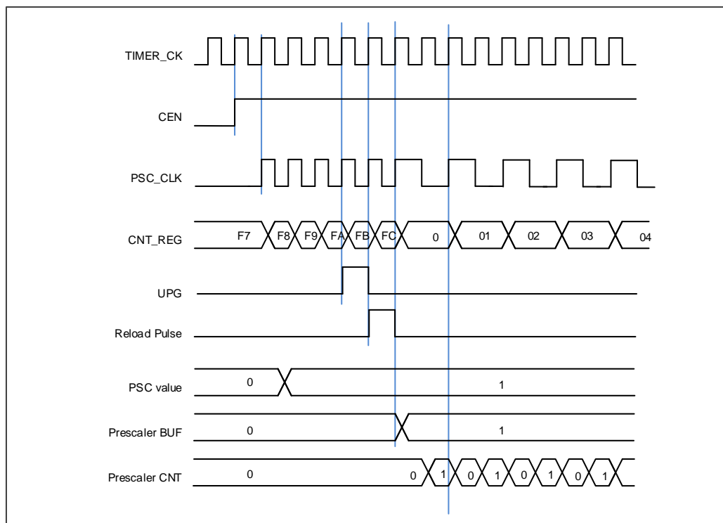
Figure 16-69. Counter timing diagram with prescaler division change from 1 to 2
