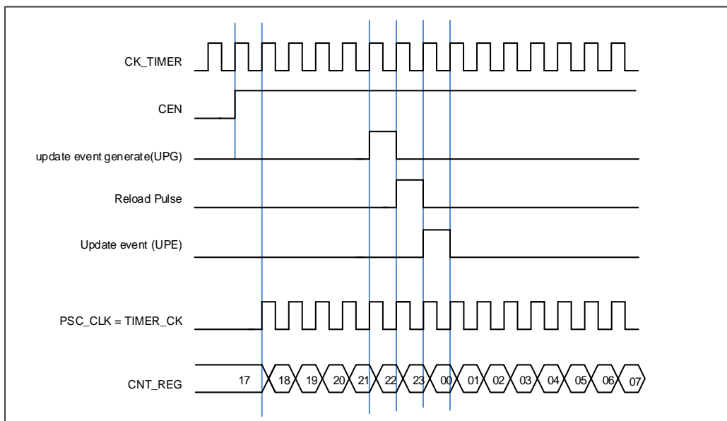
Figure 16-76. Normal mode, internal clock divided by 1
