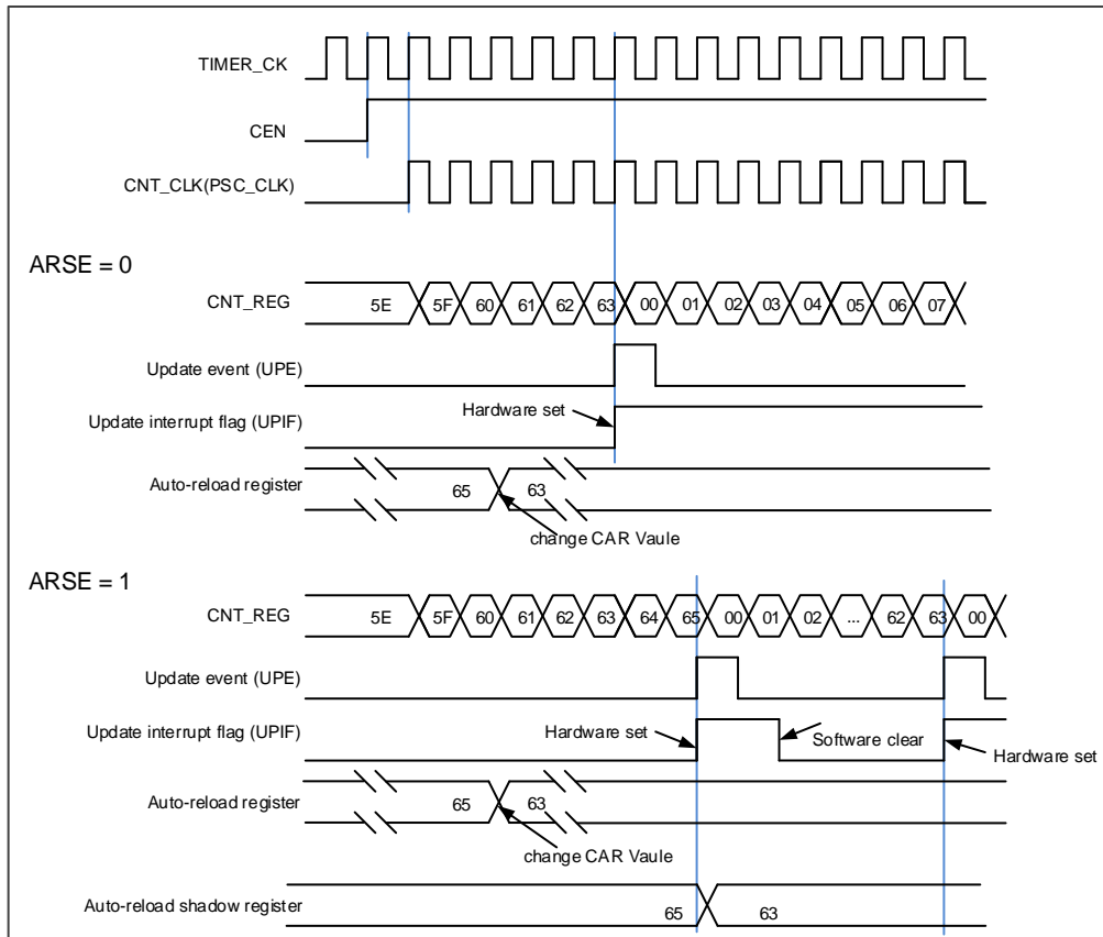
Figure 16-38. Timing chart of up counting, change TIMERx_CAR ongoing
