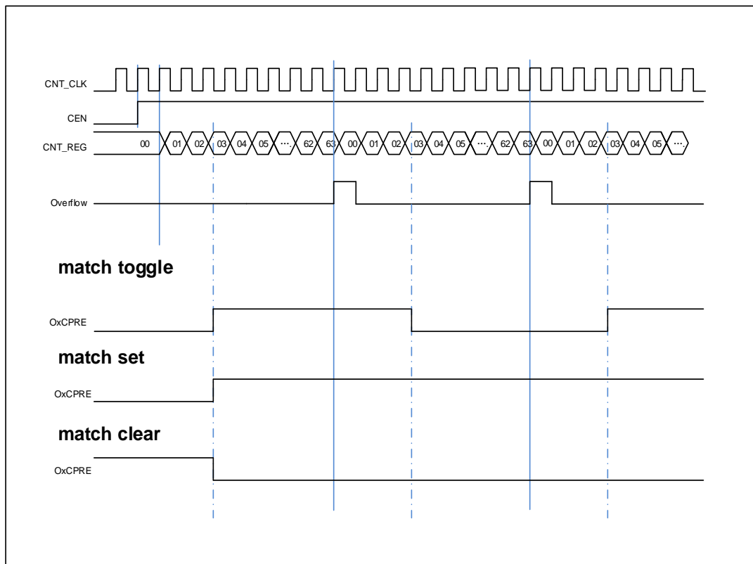
Figure 16-44. Output-compare under three modes
