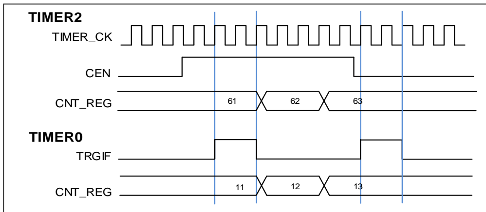
Figure 16-31. Pause mode of TIMER0 controlled by enable signal of TIMER2
