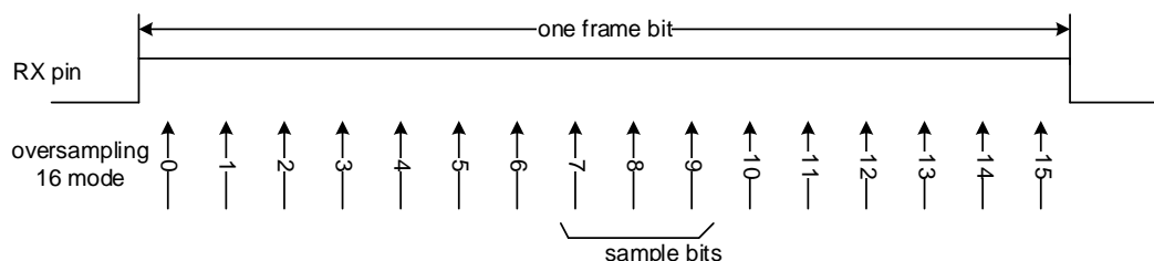
Figure 17-4. Receiving a frame bit by oversampling method
