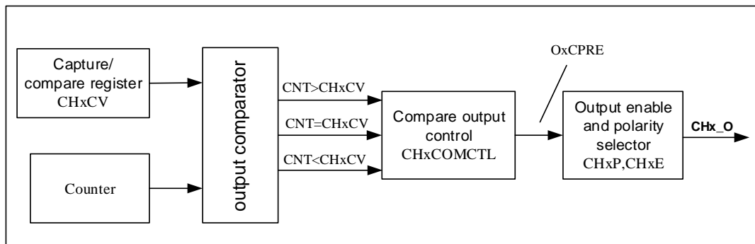
Figure 16-43. Output compare logic (x=0,1,2,3)
