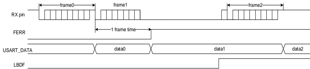
Figure 17-10. Break frame occurs during a frame
