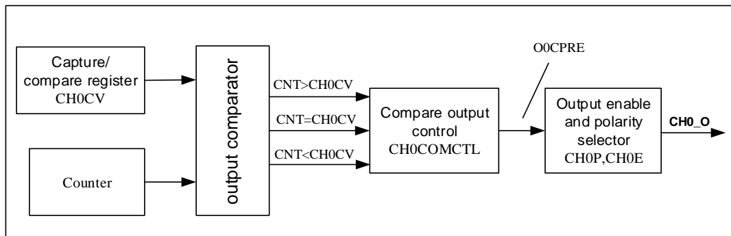
Figure 16-73. Output compare logic
