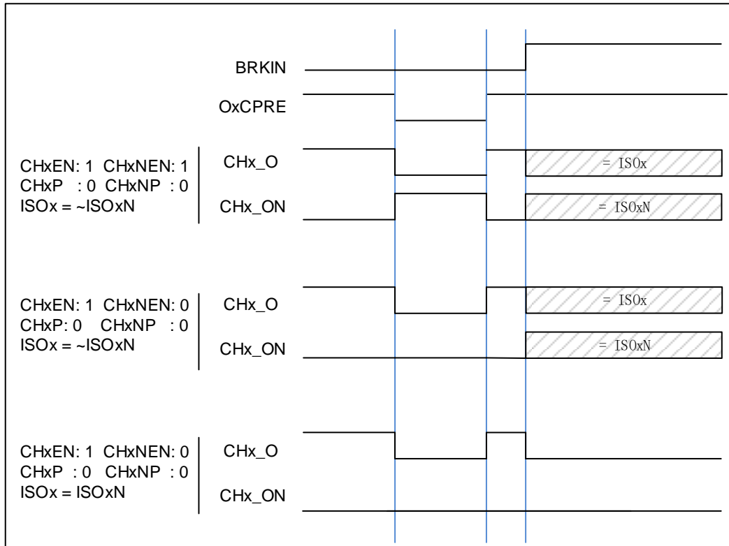
Figure 16-19. Output behavior of the channel in response to a break (the break high active)
