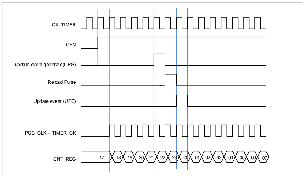
Figure 16-68. Normal mode, internal clock divided by 1
