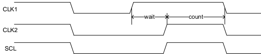
Figure 18-4. Clock synchronization
