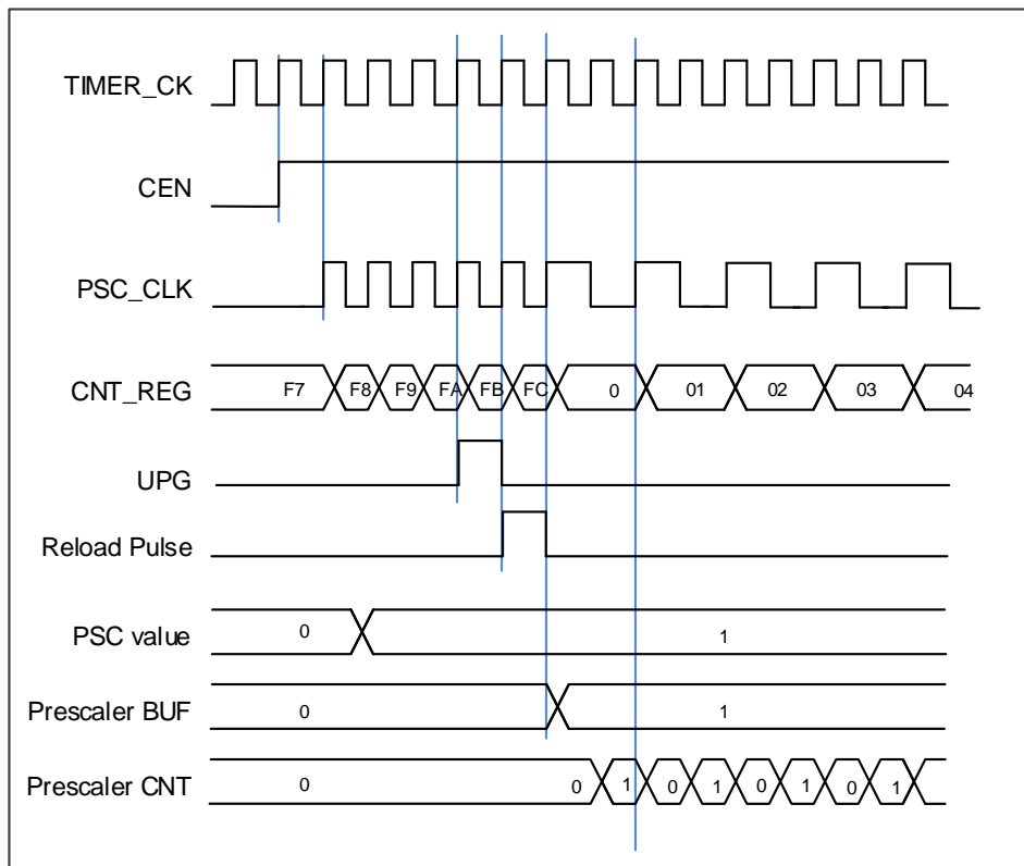
Figure 16-3. Counter timing diagram with prescaler division change from 1 to 2
