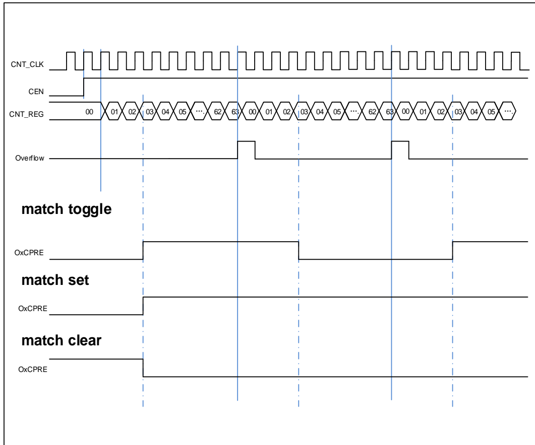
Figure 16-60. Output-compare under three modes
