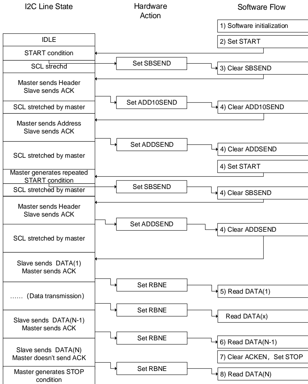
Figure 18-12. Programming model for master receiving mode using Solution A
