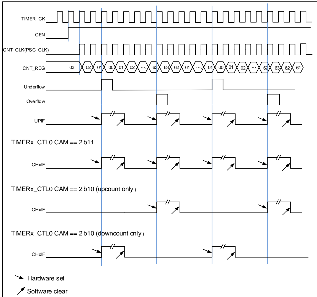
Figure 16-41. Timing chart of center-aligned counting mode
