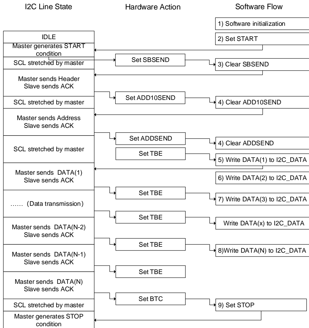
Figure 18-11. Programming model for master transmitting mode
