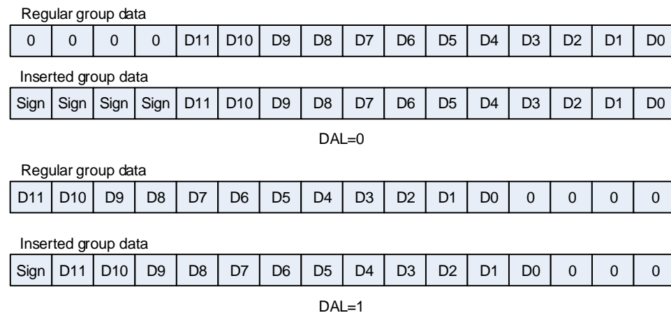
Figure 12-9. 12-bit data alignment
