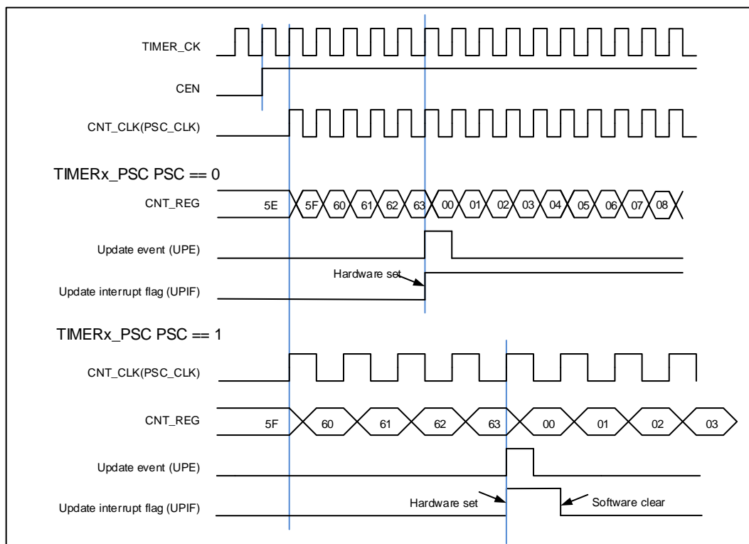
Figure 16-70. Timing chart of up counting mode, PSC=0/1
