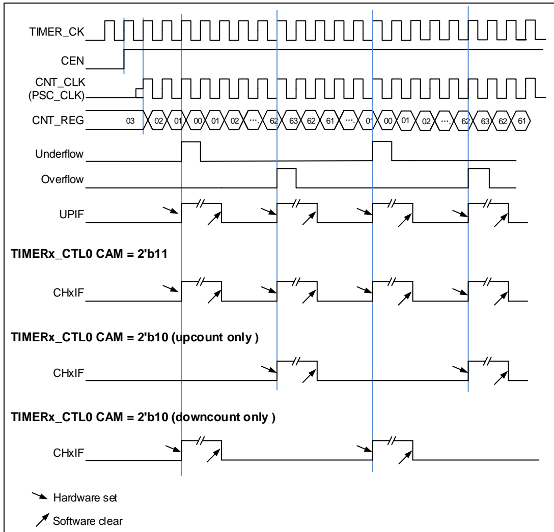
Figure 16-8. Timing chart of center-aligned counting mode
