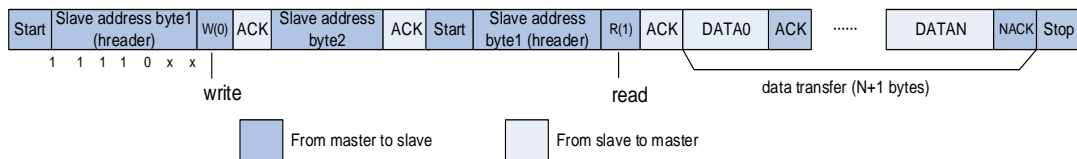
Figure 18-8. I2C communication flow with 10-bit address(Master Receive)
