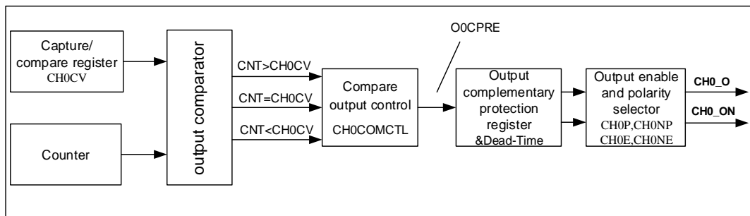
Figure 16-13. Output compare logic (with complementary output, x=0,1,2)
