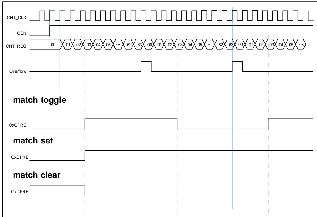
Figure 16-74. Output-compare in three modes
