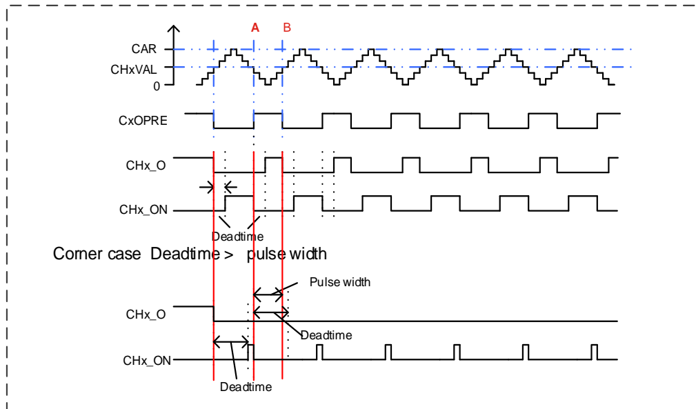
Figure 16-18. Complementary output with dead time insertion
