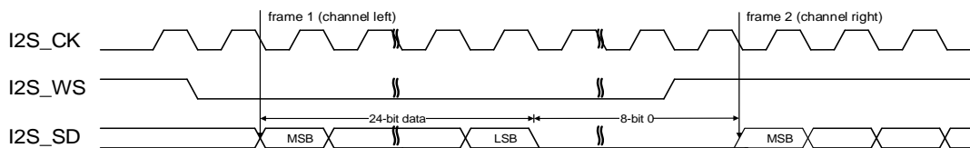
Figure 19-19. I2S Phillips standard timing diagram (DTLEN=01, CHLEN=1, CKPL=0)
