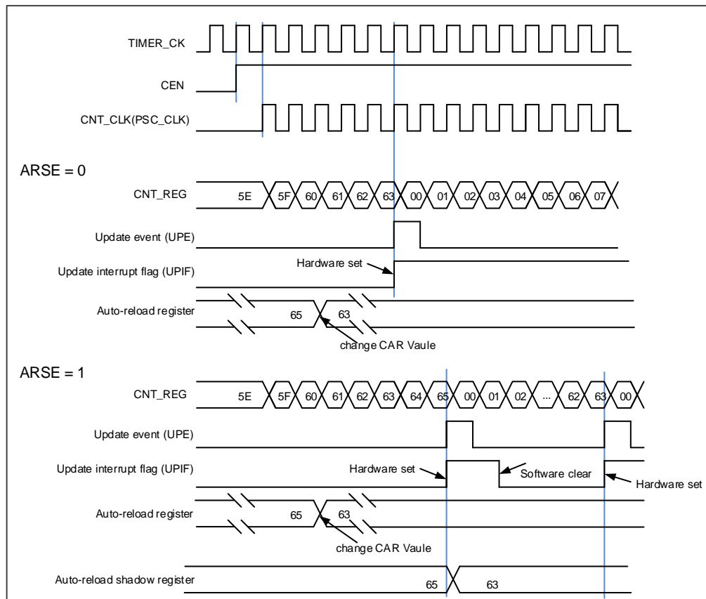
Figure 16-57. Timing chart of up counting mode, change TIMERx_CAR ongoing
