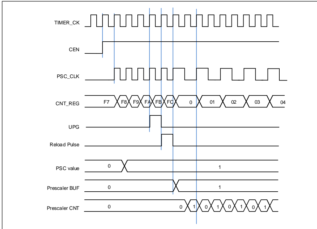
Figure 16-77. Counter timing diagram with prescaler division change from 1 to 2
