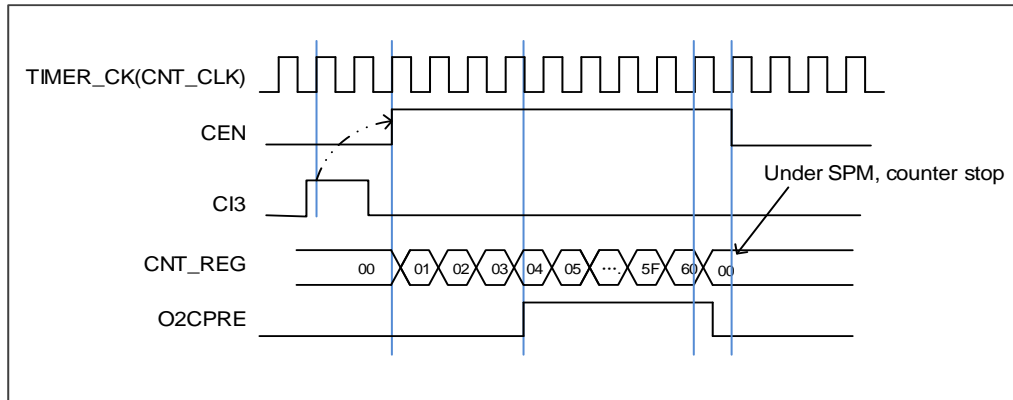
Figure 16-27. Single pulse mode TIMERx\_CHxCV=0x04 , TIMERx\_CAR=0x60
