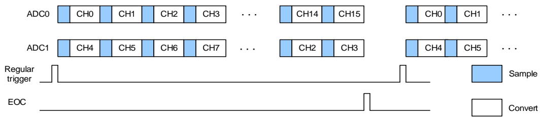
Figure 12-14. Regular parallel mode on 16 channels
