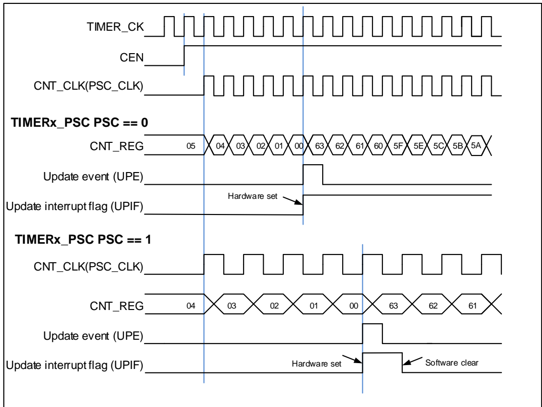
Figure 16-6. Timing chart of down counting mode, PSC=0/1
