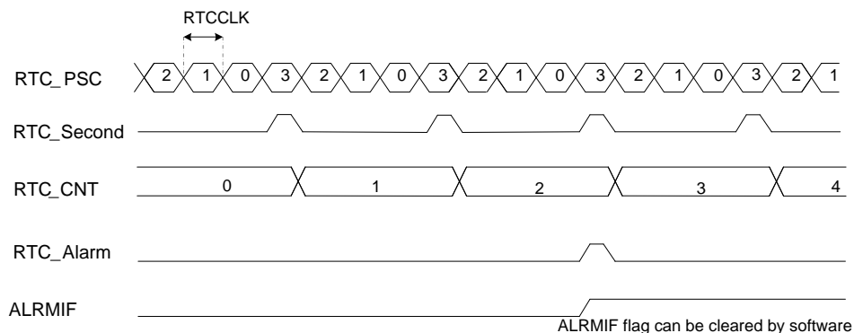
Figure 15-2. RTC second and alarm waveform example (RTC_PSC = 3, RTC_ALARM = 2)
