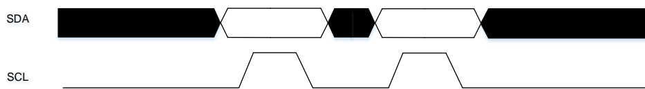
Figure 18-2. Data validation
