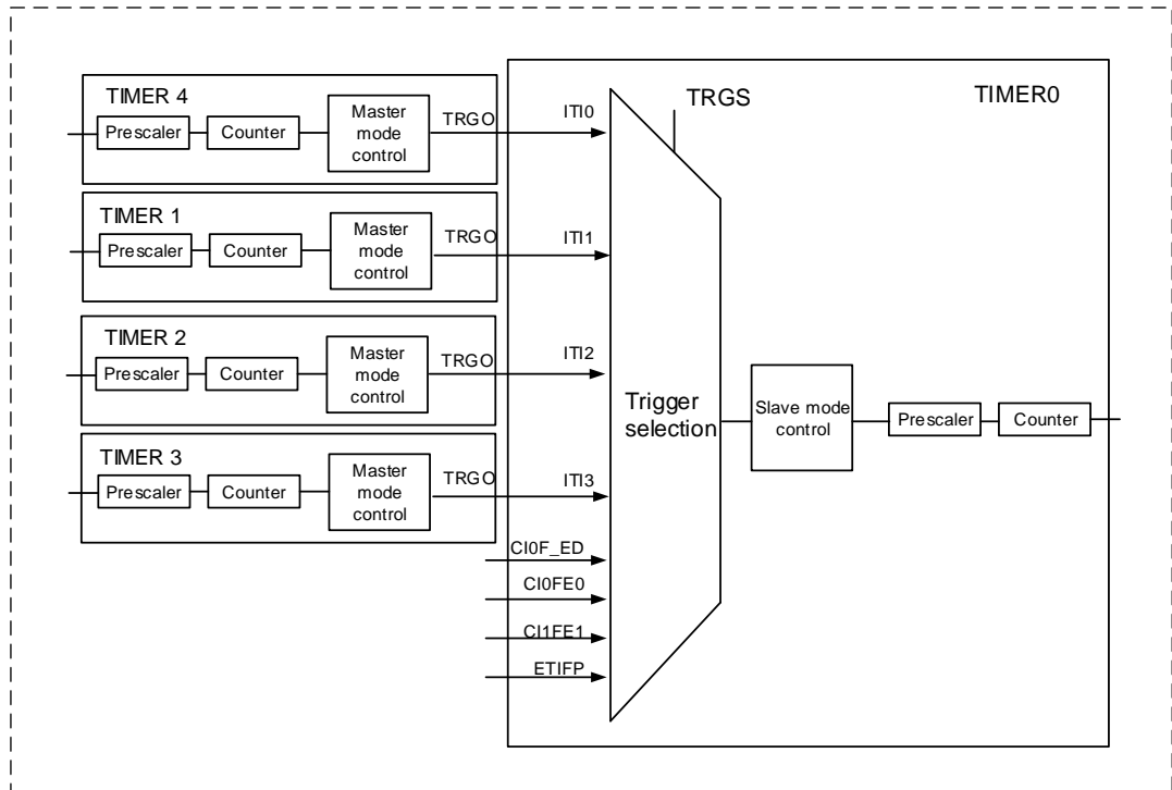
Figure 16-28. TIMER0 master/slave mode example
