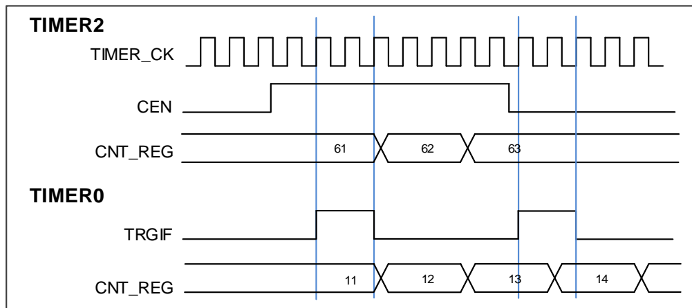
Figure 16-29. Trigger mode of TIMER0 controlled by enable signal of TIMER2
