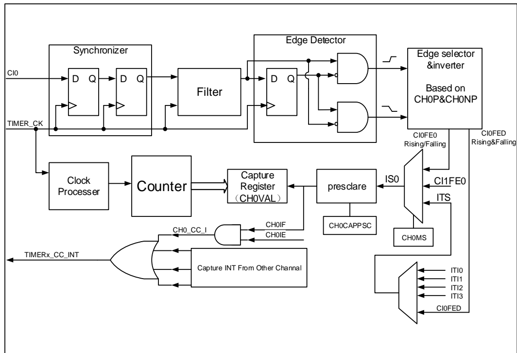
Figure 16-72. Input capture logic
