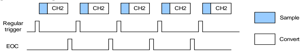
Figure 12-2. Single conversion mode
