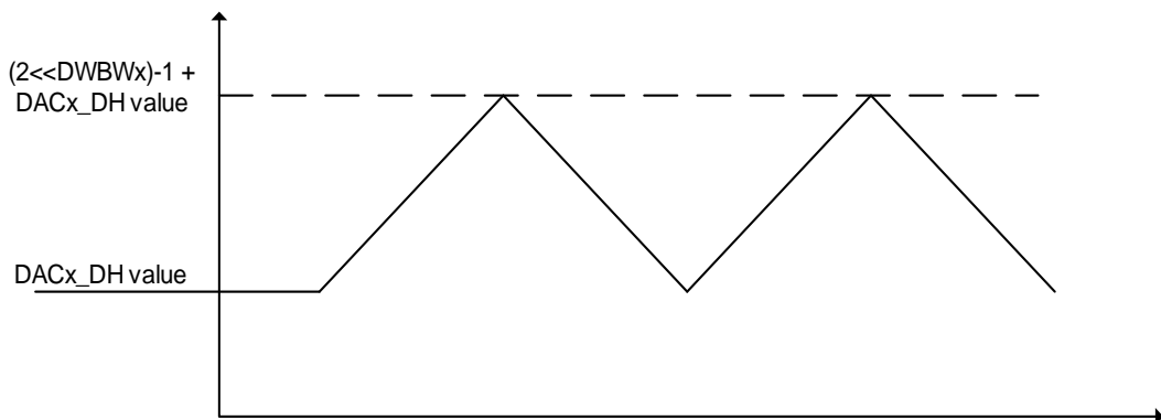
Figure 13-3. DAC triangle noise wave
