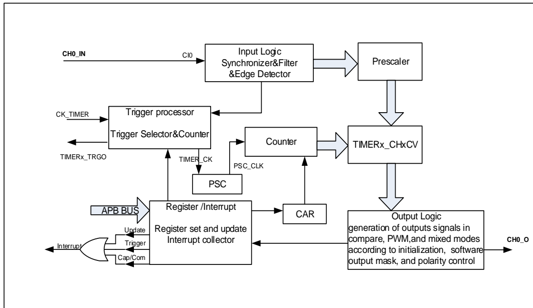
Figure 16-67. General level2 timer block diagram
