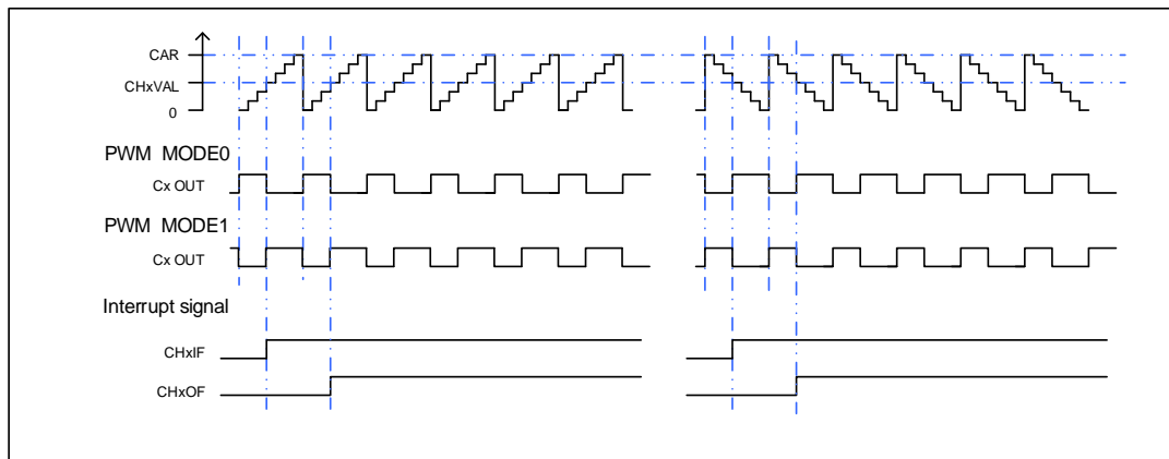
Figure 16-45. Timing chart of EAPWM
