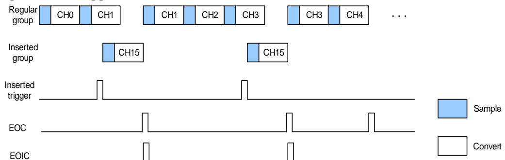
Figure 12-8. Triggered insertion
