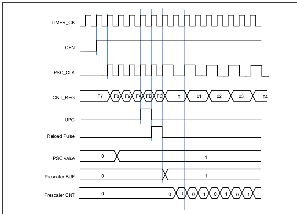
Figure 16-36. Counter timing diagram with prescaler division change from 1 to 2
