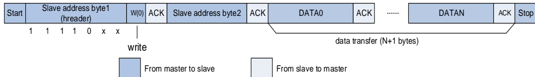
Figure 18-7. I2C communication flow with 10-bit address(Master Transmit)
