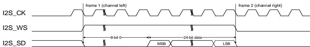
Figure 19-31. LSB justified standard timing diagram (DTLEN=01, CHLEN=1, CKPL=0)
