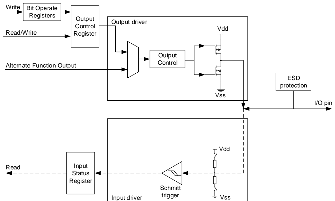
Figure 8-3. Output configuration
