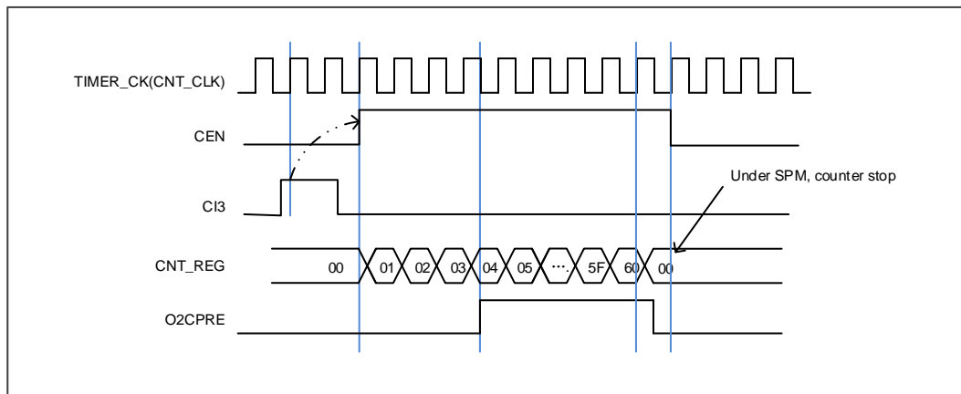
Figure 16-66. Single pulse mode TIMERx\_CHxCV = 0x04 , TIMERx\_CAR=0x60
