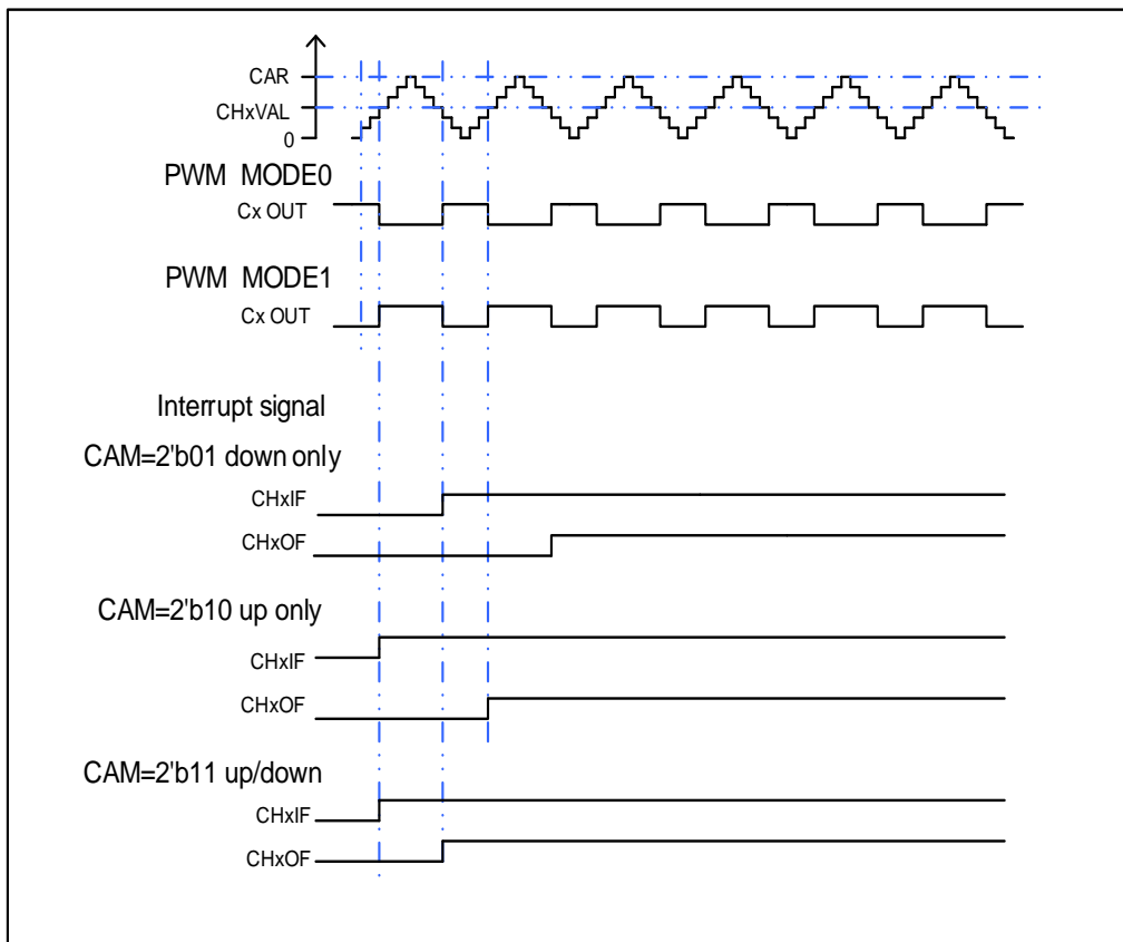
Figure 16-62. Timing chart of CAPWM
