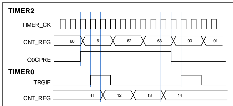
Figure 16-32. Pause mode of TIMER0 controlled by O0CPREF signal of TIMER2
