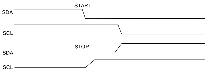
Figure 18-3. START and STOP condition
