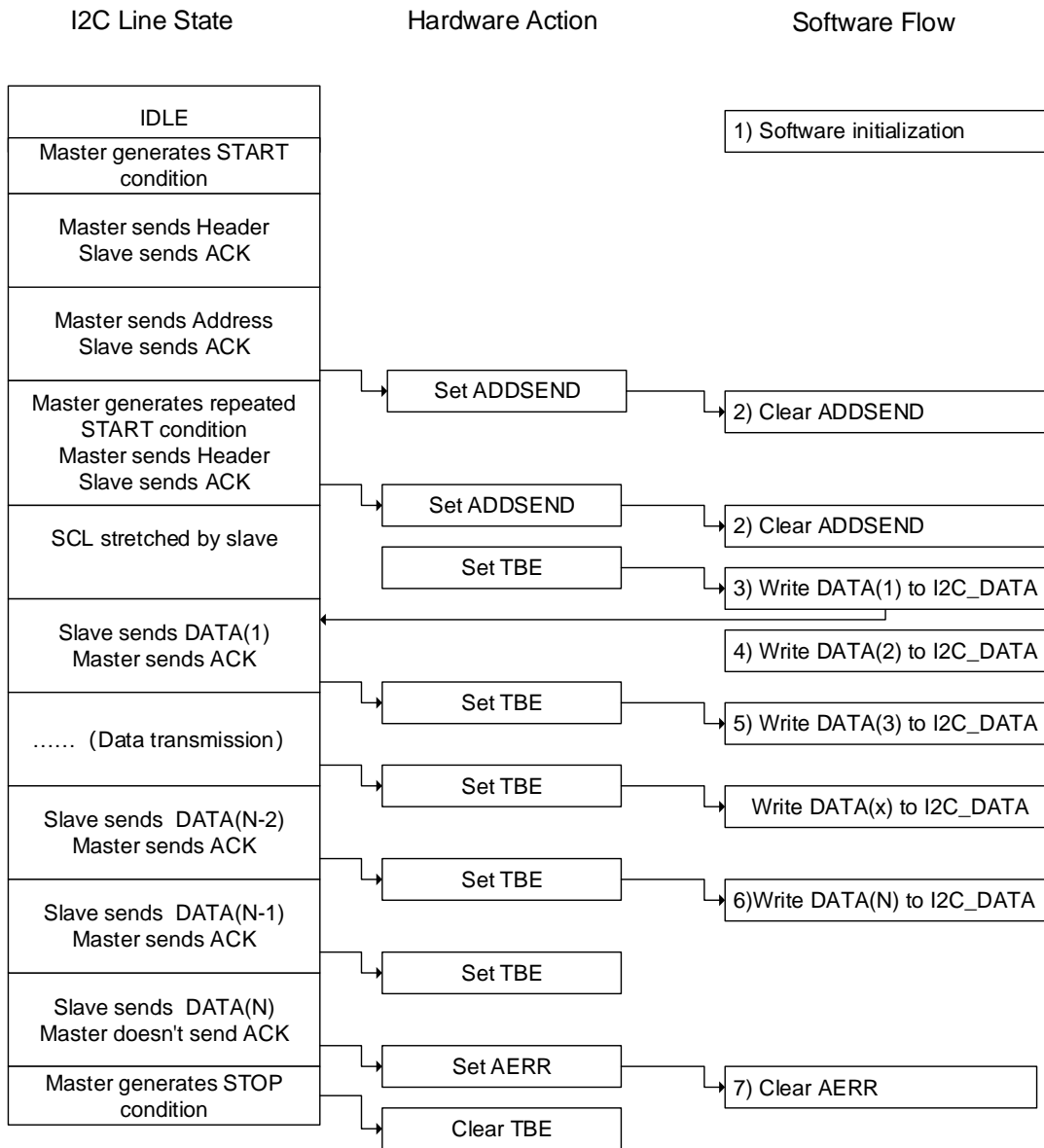
Figure 18-9. Programming model for slave transmitting mode
