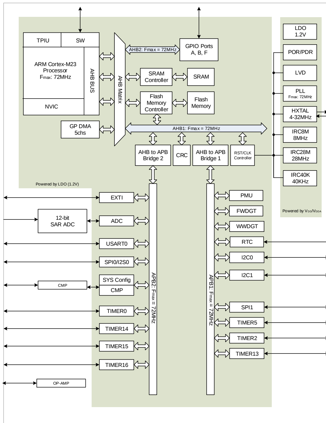
Figure 2-1. GD32E231K8Q6 block diagram
