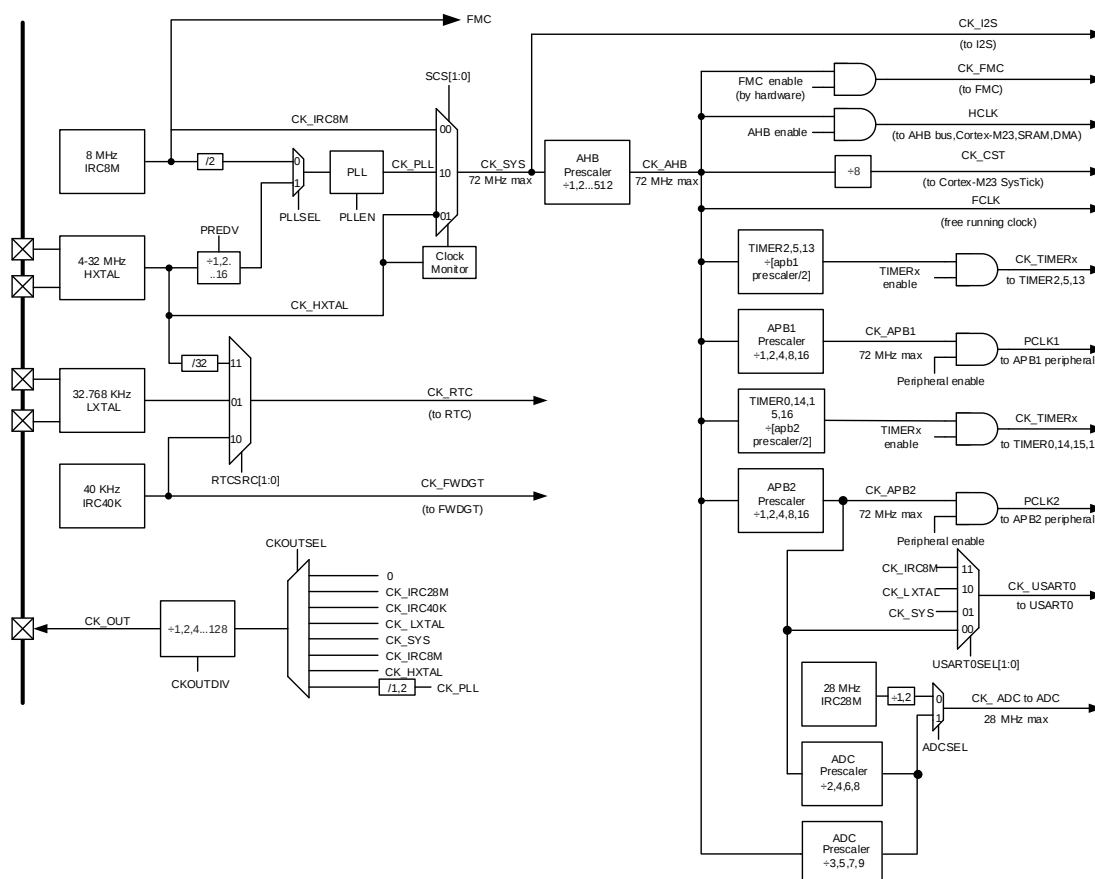
Figure 2-3. GD32E231K8Q6 clock tree
