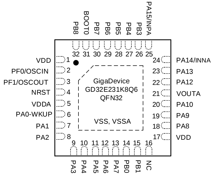
Figure 2-2. GD32E231K8Q6 QFN32 pinouts
