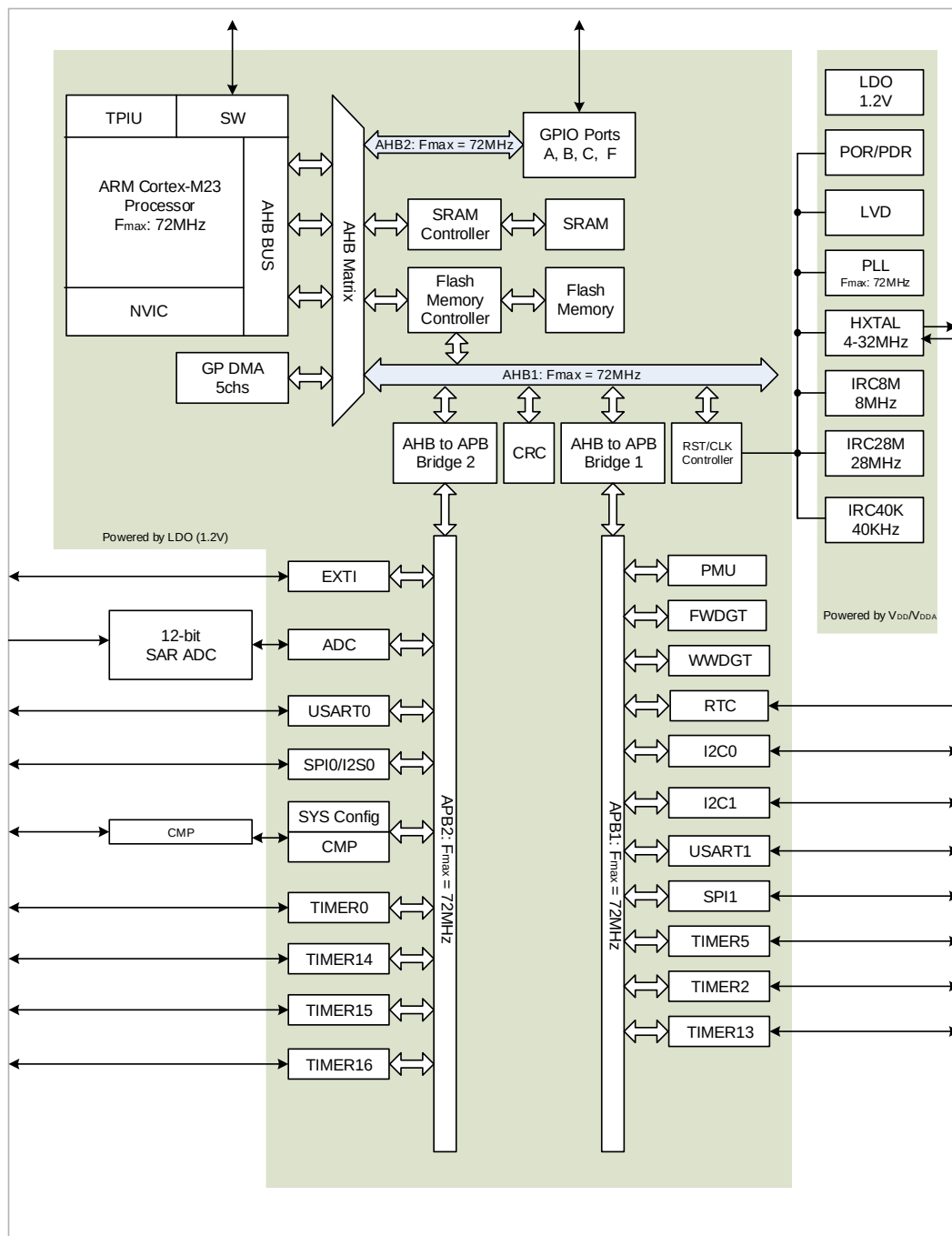
Figure 2-1. GD32E235xx block diagram
