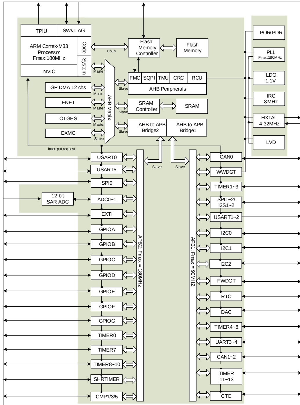
Figure 2-1. GD32E508xx block diagram
