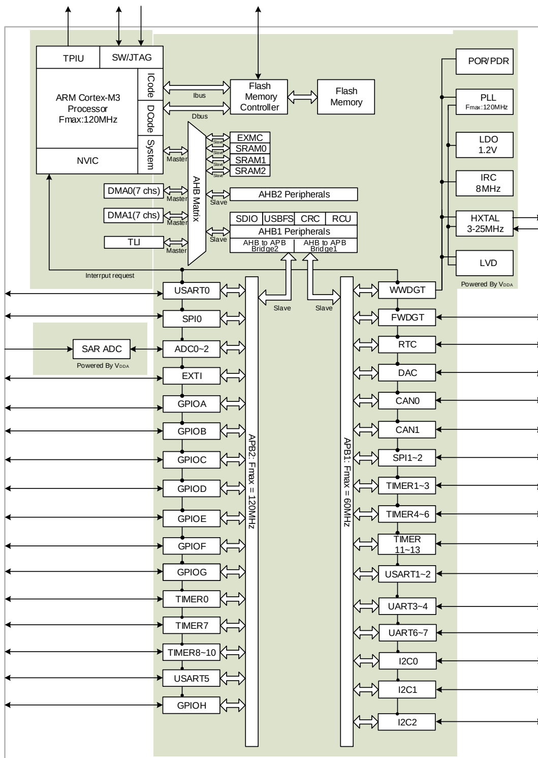
Figure 2-1. GD32F205xx block diagram
