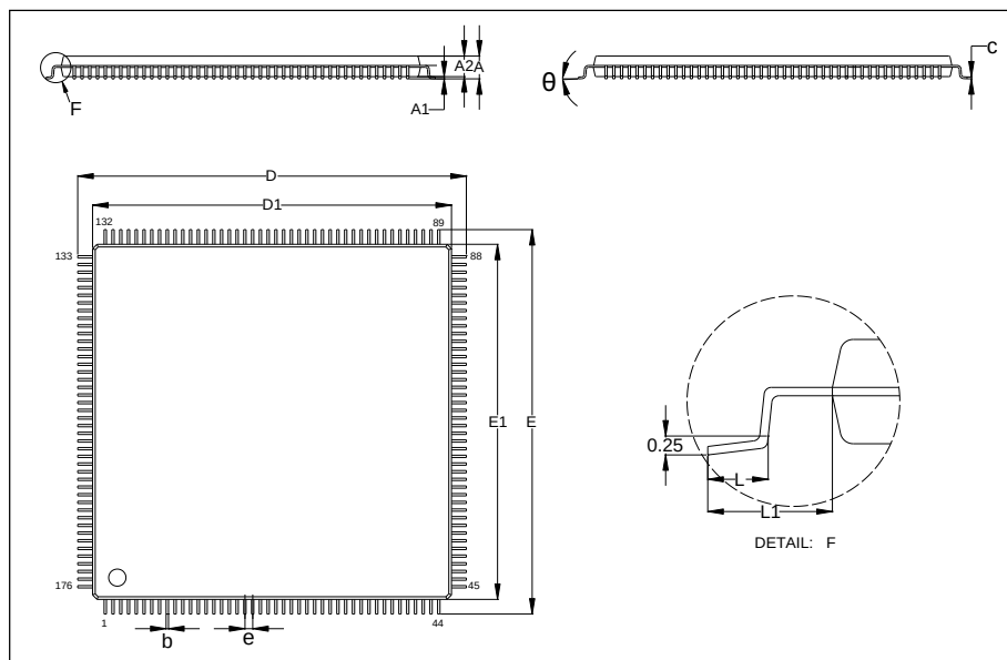
Figure 5-1. LQFP176 package outline
