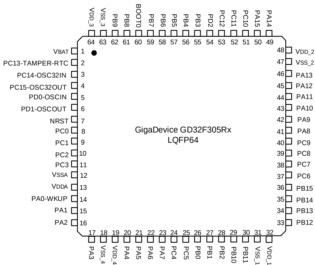
Figure 2-4. GD32F305Rx LQFP64 pinouts
