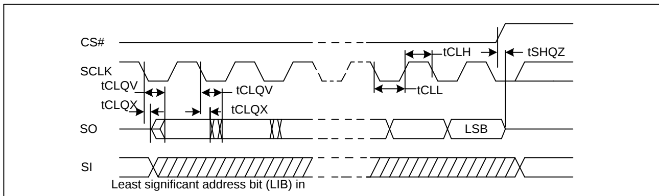
Figure 98. Output Timing
