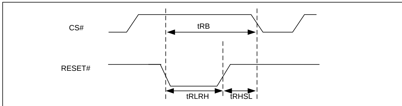
Figure 101. RESET Timing
