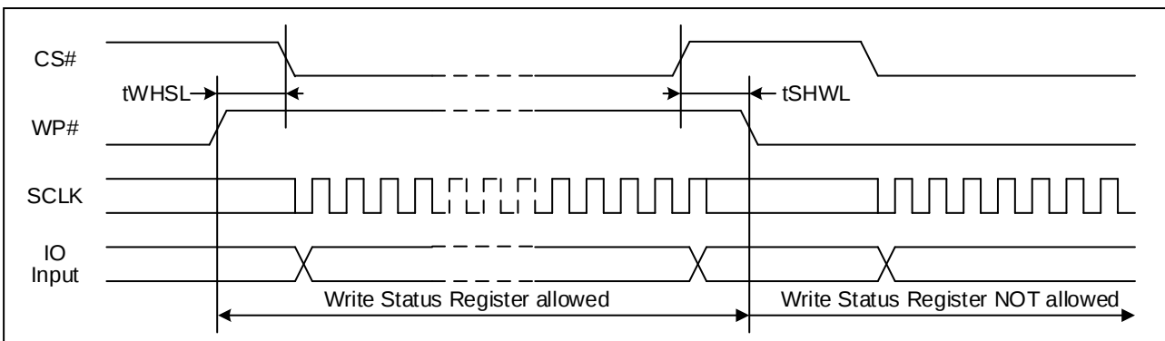
Figure 102. WP# Timing
