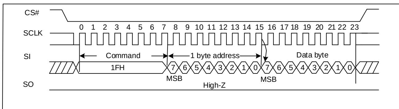
Figure12-2. Set Features Timing Diagram
