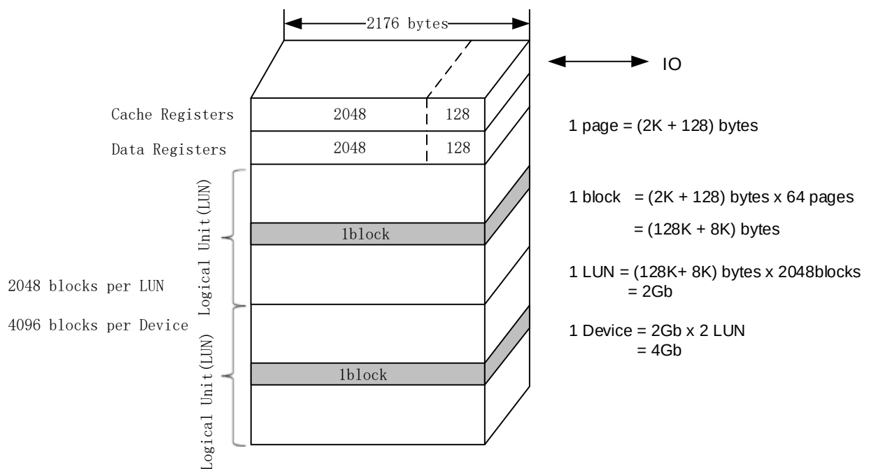
Figure 3-1.Array Organization
