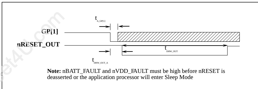
Figure 6. GPIO Reset Timing
