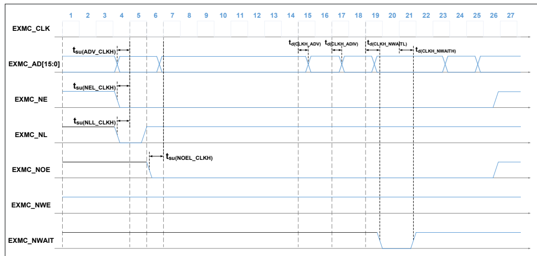
Figure 4-14. Synchronous multiplexed read timings diagram
