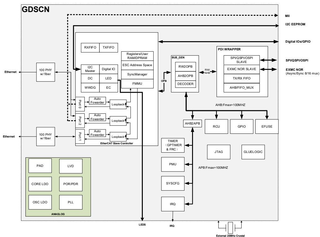
Figure 2-2. GDSCN block diagram
