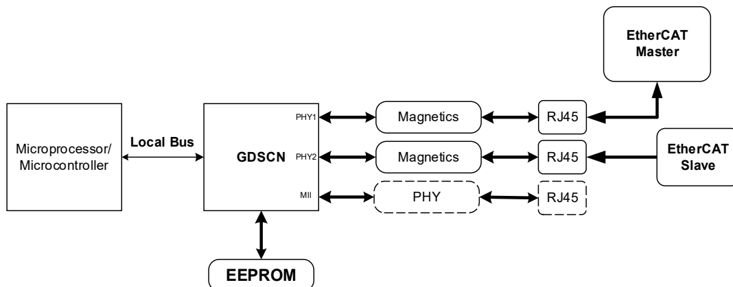
Figure 2-1. GDSCN system diagram
