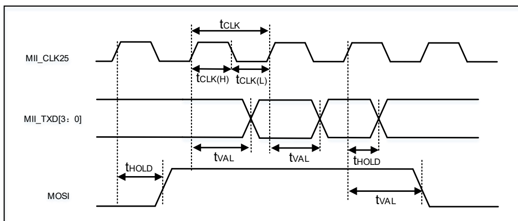
Figure 4-16. MII TX timing diagram
