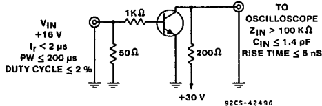
Fig. 3—Turn-on time test circuit for npn types (2221A and 2222A).
