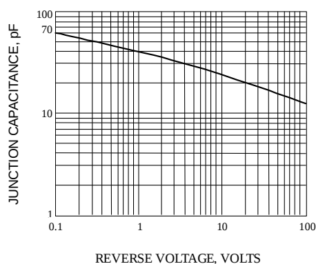
Fig. 6-TYPICAL JUNCTION CAPACITANCE
