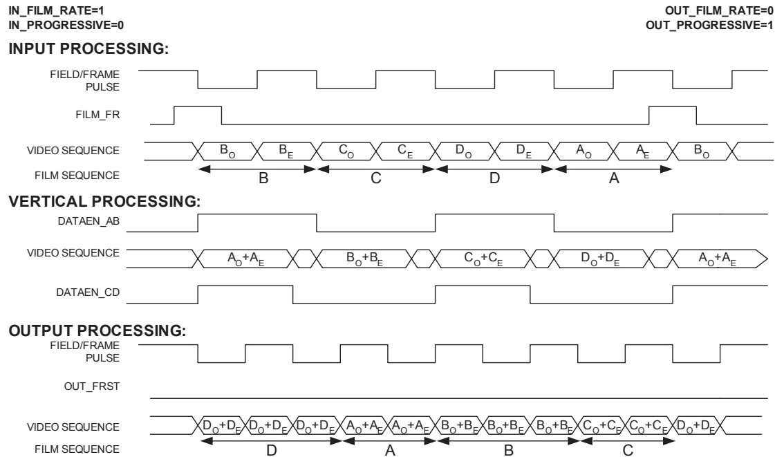
Figure 3-31: 24i/24p/60p Processing
