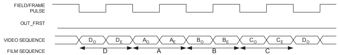
Figure 3-16: 30i/24p/24i Processing
