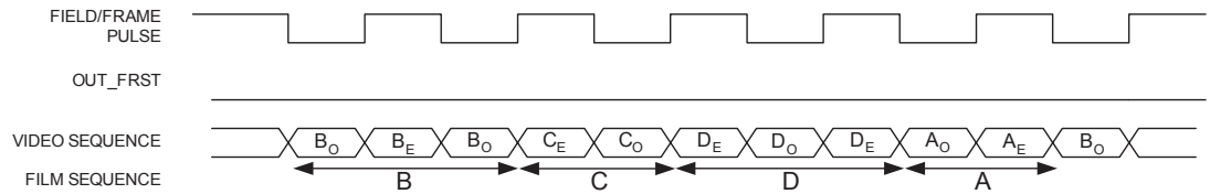
Figure 3-36: 24p/24p/30i Processing
