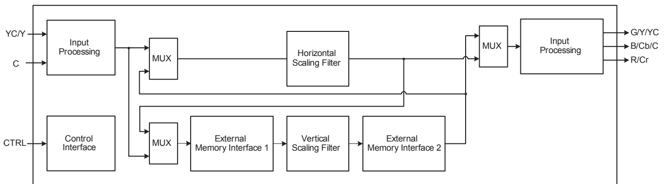
Block Diagram
