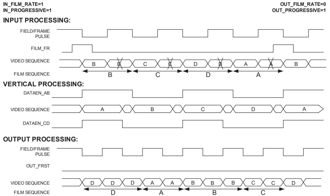
Figure 3-30: 48p/24p/60p Processing
