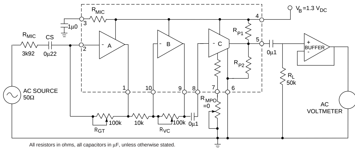
Fig. 5 Characterization Circuit
