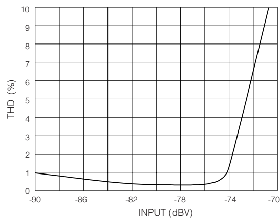
Fig. 9 Distortion vs Input Level ( R_{GT} = R_{VC} = 100k )
