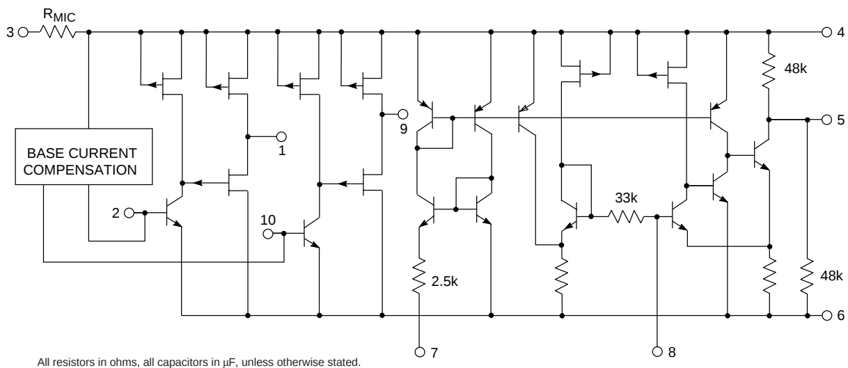
Fig. 2 Functional Schematic
