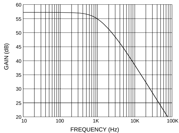
Fig. 10 Preamplifier Open Loop Frequency Response
