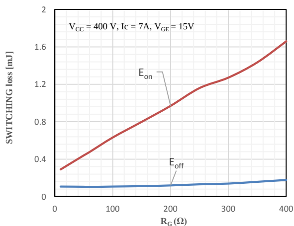
Fig 11 Switching Loss vs. Gate Resistor
