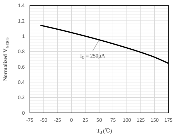
Fig 4 Normalized V_{GE(th)} vs. Junction Temperature
