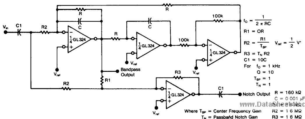
Figure 5 — Bi-Quad Filter
