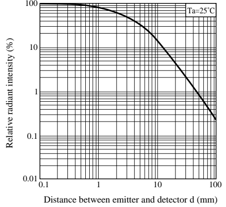
Fig. 9 GL4600 Relative Radiant Intensity vs. Distance (Detector : PT4600)
