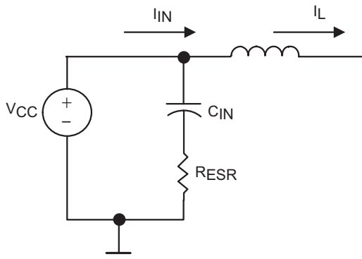
Figure 11. Boost Circuit Effective Input Filter
