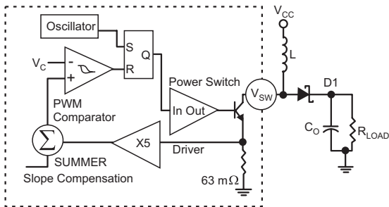
Figure 6. Current Mode Control Scheme
