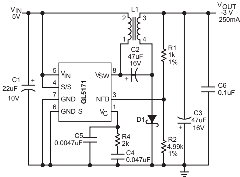
Figure 26. Low Ripple 5V to -3V "Cuk" Converter
