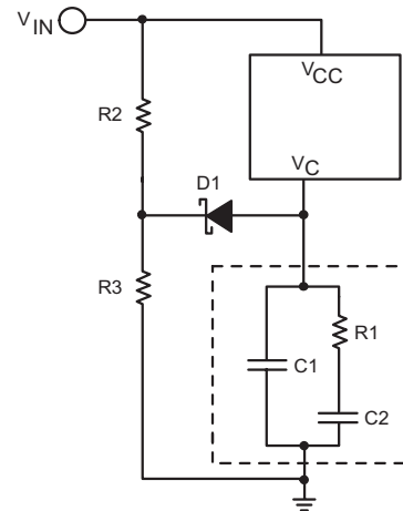
Figure 12. Current Limiting using a Diode Clamp
