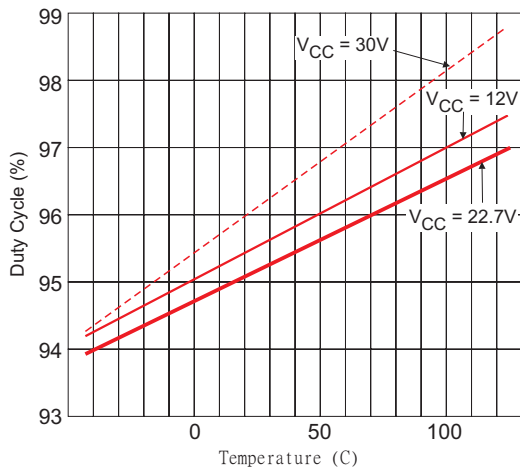
Figure 5. Maximum Duty Cycle vs. Temperature
