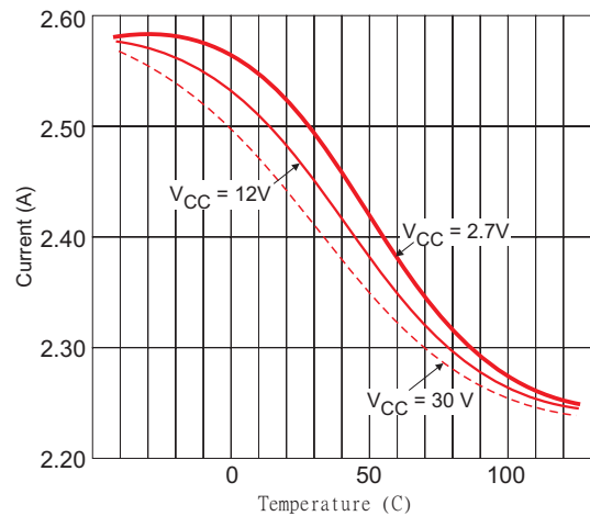
Figure 4. Current Limit vs. Temperature
