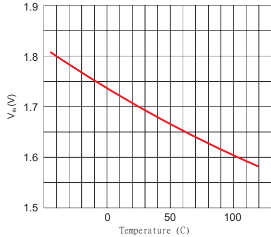
Figure 2. Minimum Input Voltage vs. Temperature
