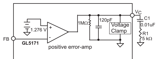
Figure 8. Error Amplifier Equivalent Circuit
