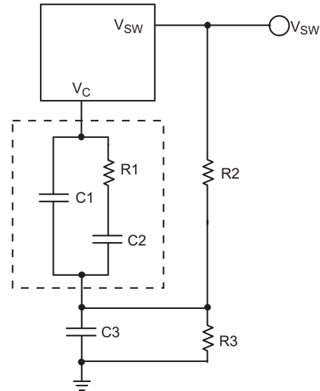
Figure 14. Technique for Increasing Slope Compensation
