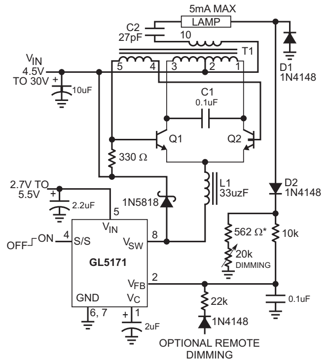
Figure 27. CCFL Supply
