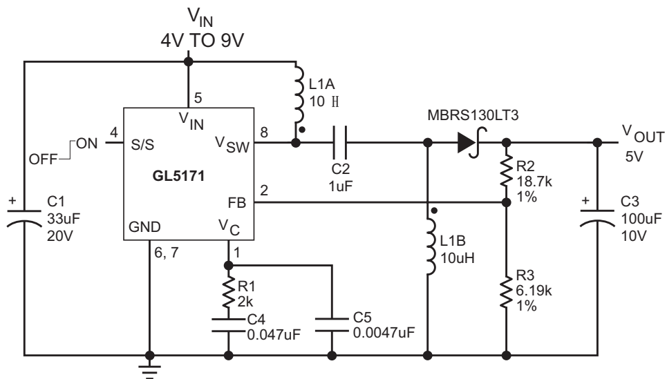
Figure 28. 2 Li - Lion Cell to 5V SEPIC Converter
