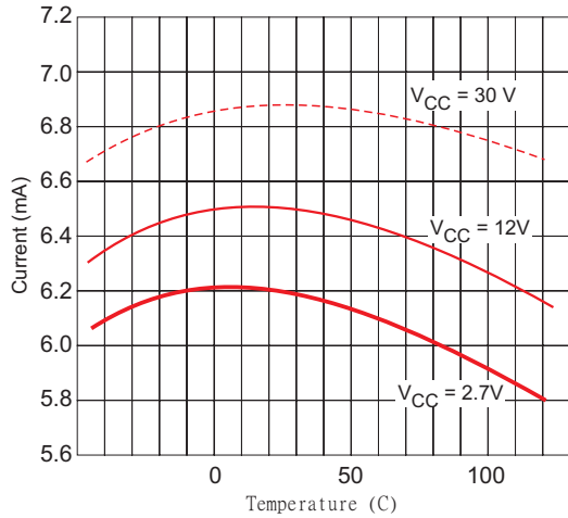
Figure 1. I CC (No Switching) vs. Temperature
