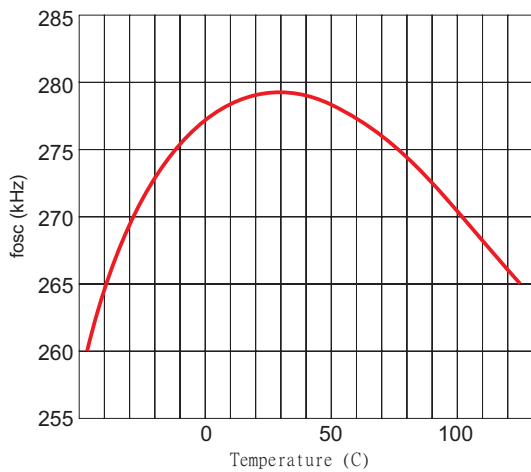
Figure 3. Switching Frequency vs. Temperature (GL5171 ONLY)
