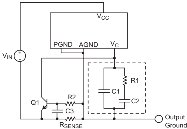
Figure 13. Current Limiting using a Current Sense Resistor
