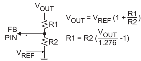
Figure 16. Output Resistor Divider
