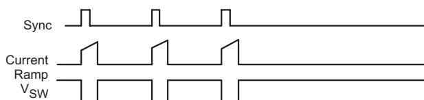
Figure 7. Timing Diagram of sync and shutdown
