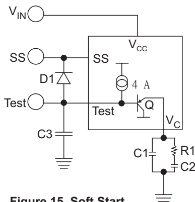
Figure 15. Soft Start
