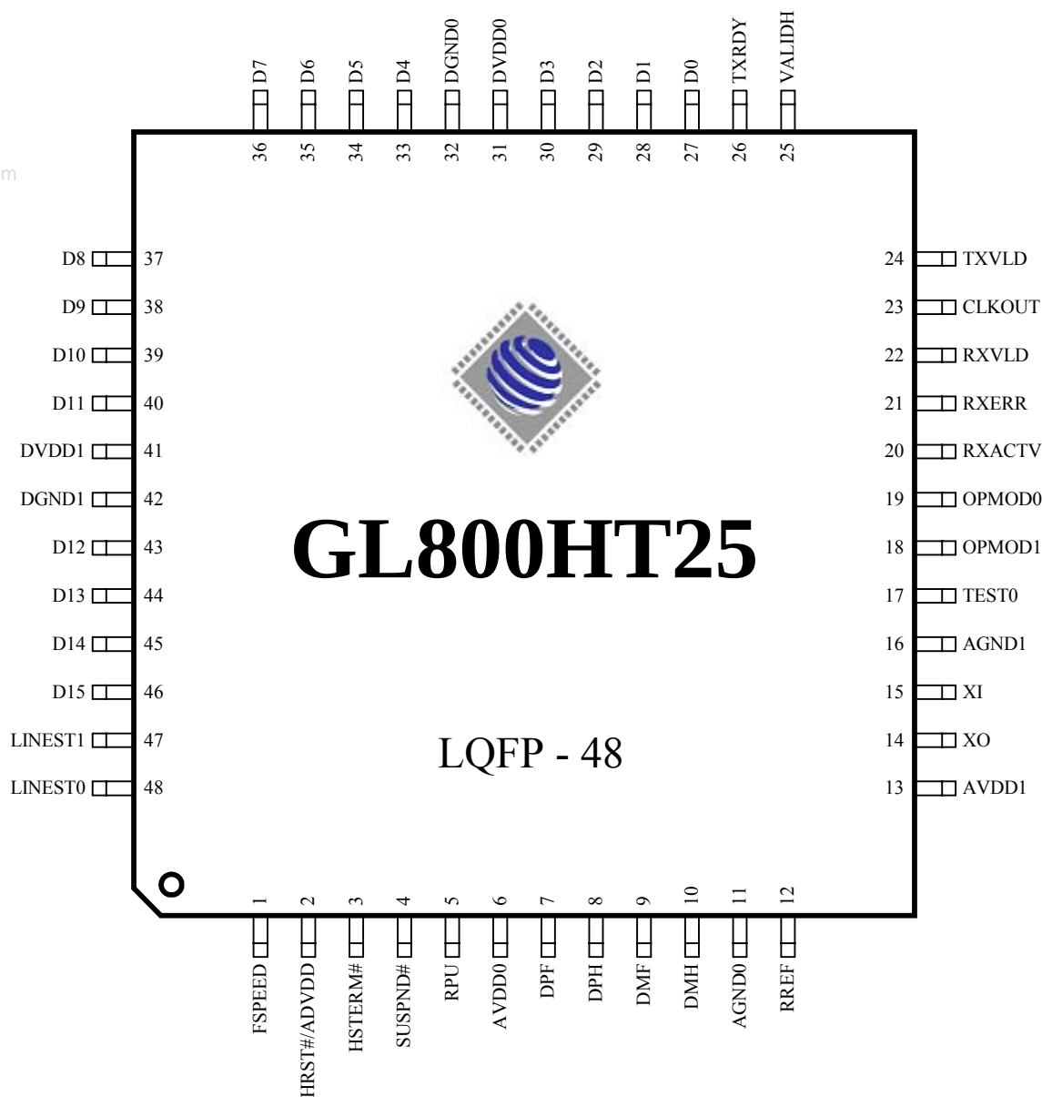
Figure 4.1 - Pinout Diagram
