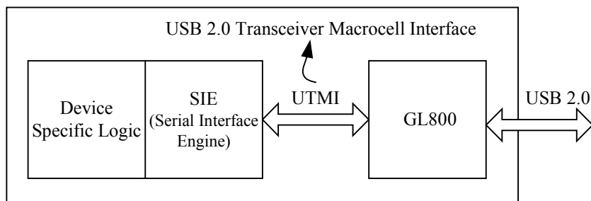
Figure 3.1 - System Diagram
