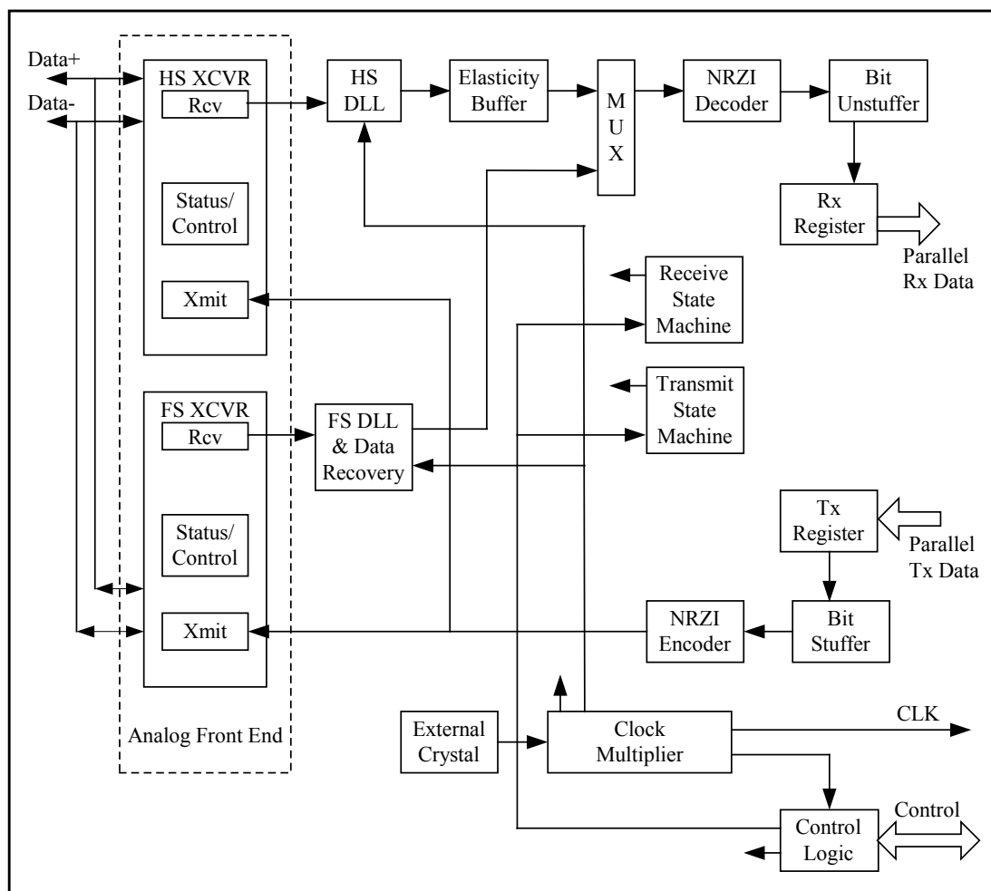
Figure 3.2 - Block Diagram
