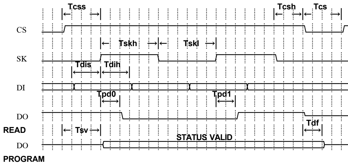
Figure 6.9 - Timing Diagram of 93C46
