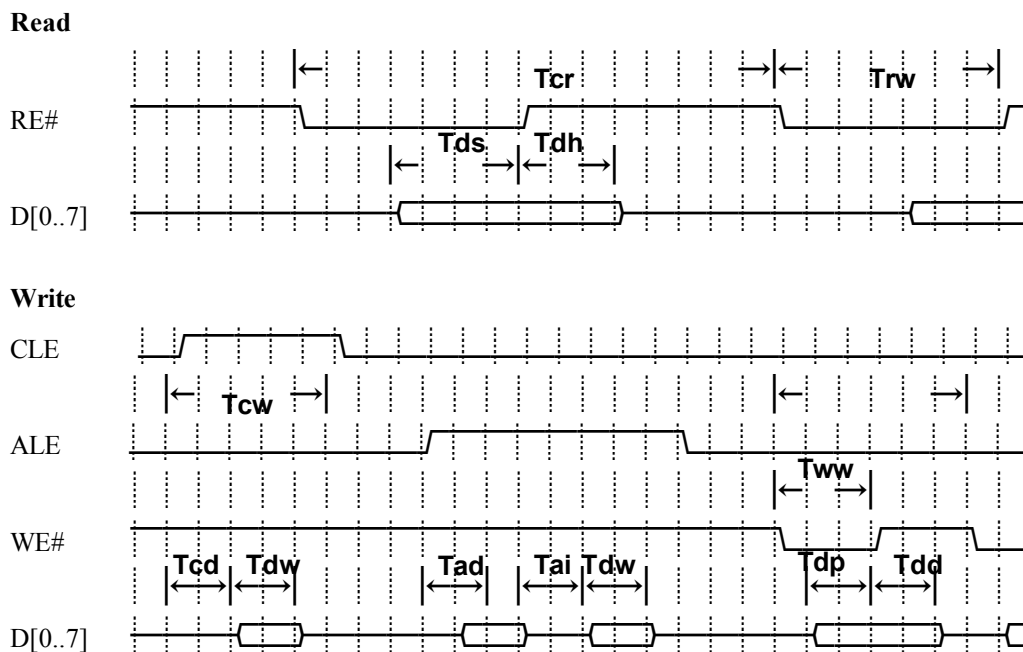
Figure 6.2 - Timing Diagram of SmartMedia
