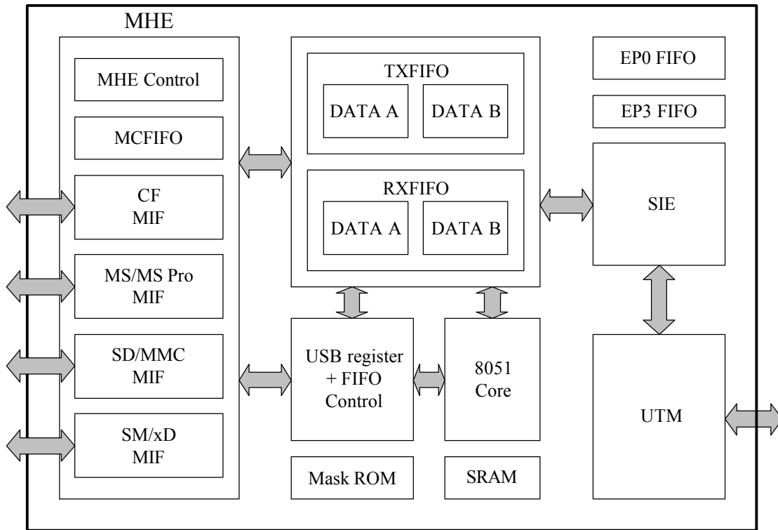
Figure 4.1 - Block Diagram
