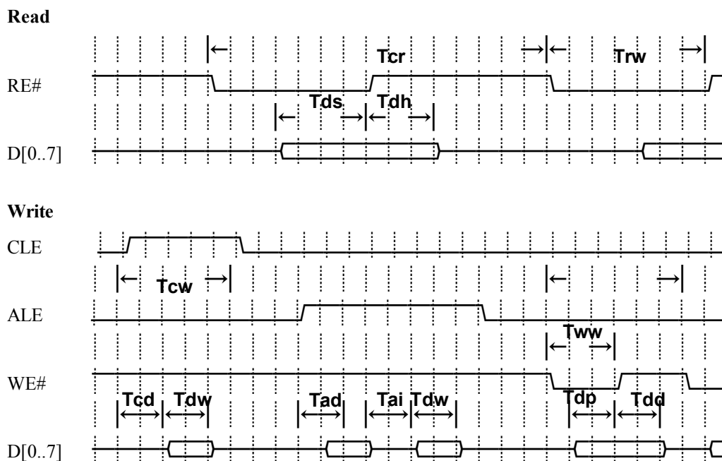
Figure 6.3 - Timing Diagram of xD-Picture
