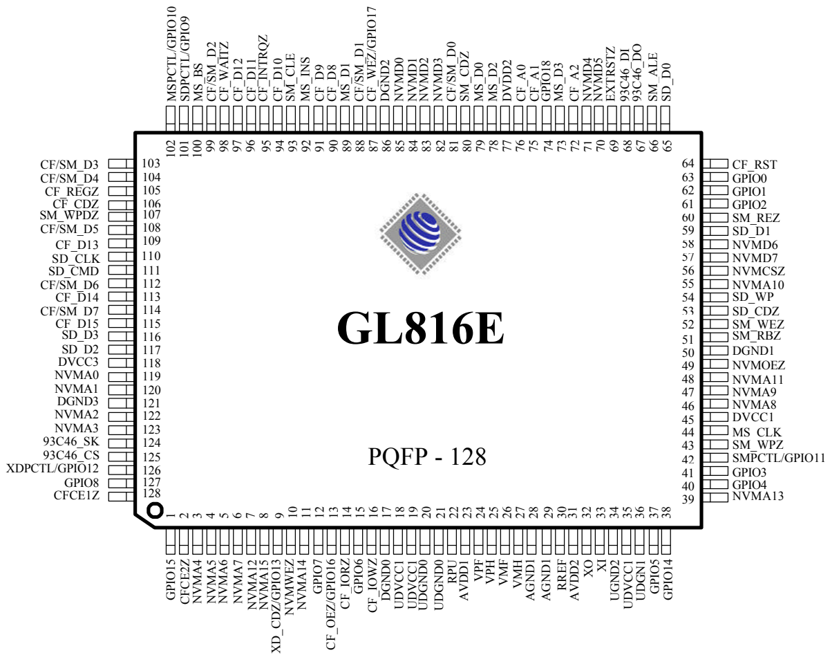
Figure 3.2 - 128 Pin PQFP Pinout Diagram
