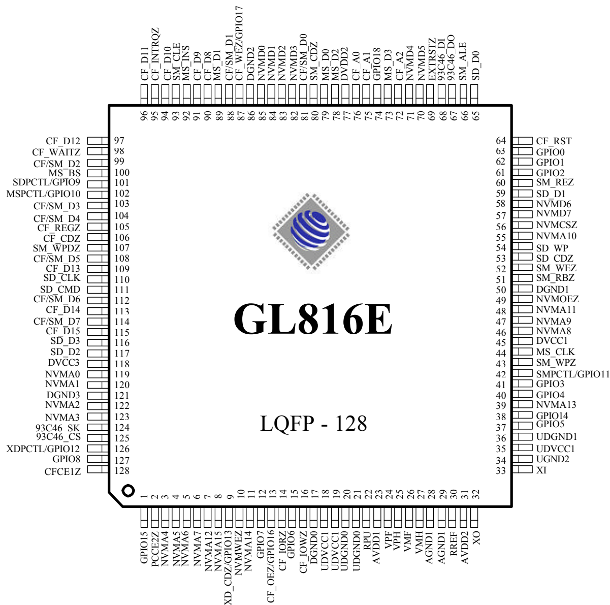
Figure 3.1 - 128 Pin LQFP Pinout Diagram
