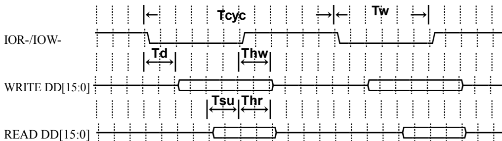
Figure 6.7 - Timing Diagram of CompactFlash
