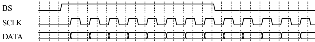
Figure 6.5 - Timing Diagram of MemoryStick PRO
