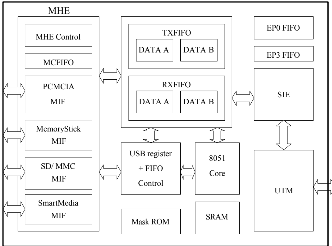
Figure 3.1 - Block Diagram
