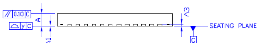
Figure 7.2 - GL860A 48 Pin LQFN Package
