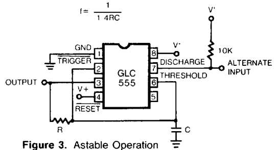
Figure 3. Astable Operation
