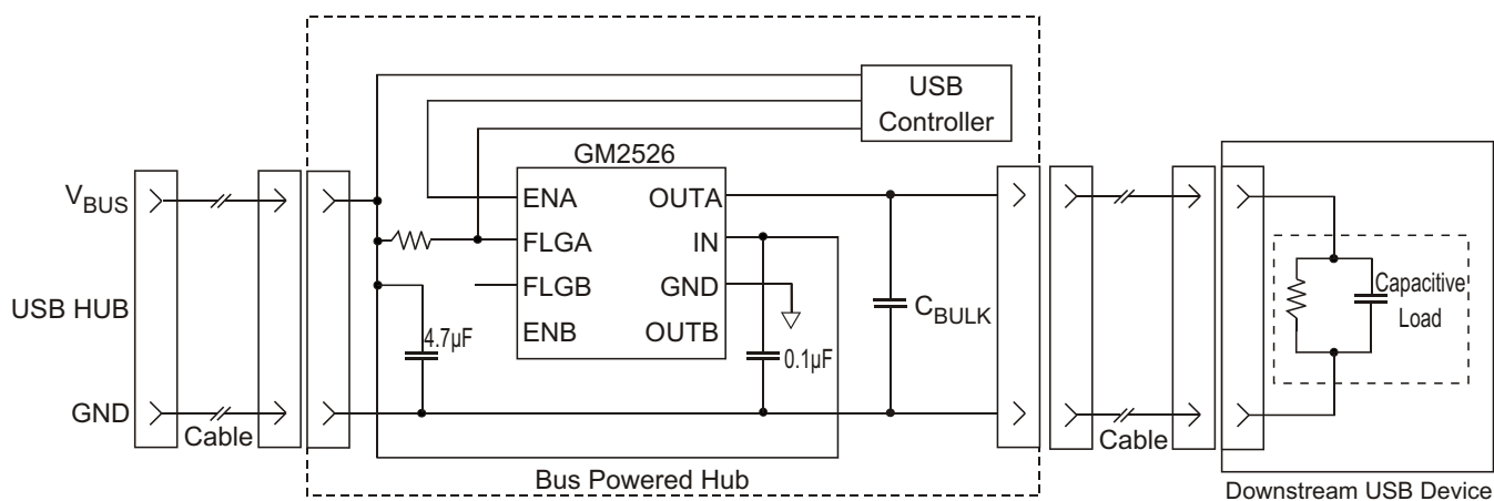
Figure 3. SOFT START (Single Channel)
