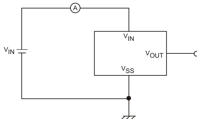
Circuit 2
