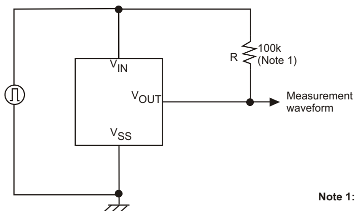
Circuit 5
