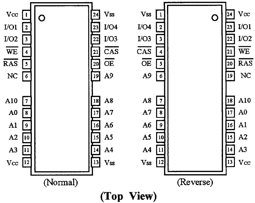
24 (26) TSOP II
