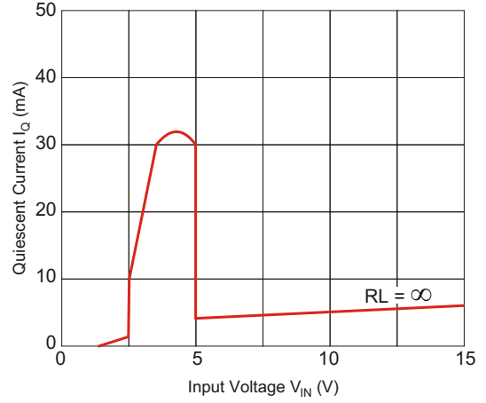
Figure 2. Quiescent Current vs. Input Voltage
