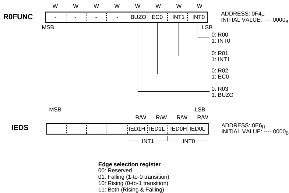
Figure 16-9 R0FUNC and IEDS Registers
