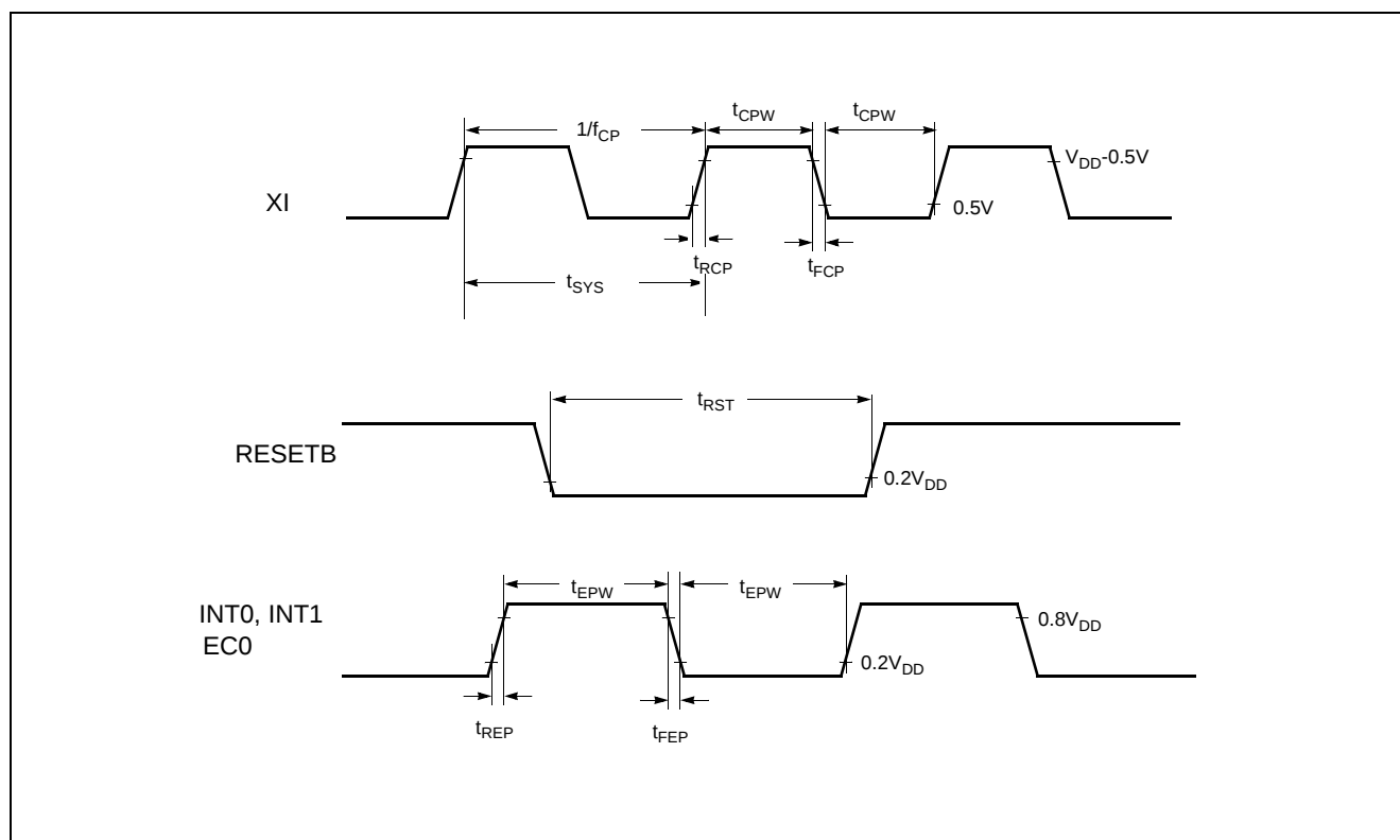
Figure 7-1 Timing Chart
