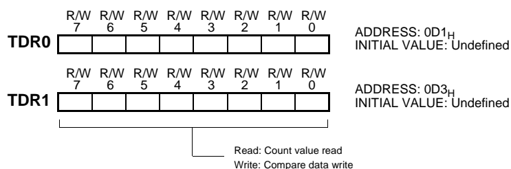
Figure 12-1 TM0, TM1 Registers
