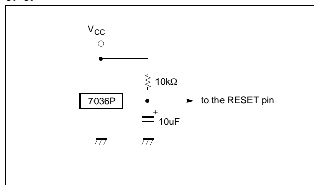
Figure 19-1 Simple Power-on-Reset Circuit
