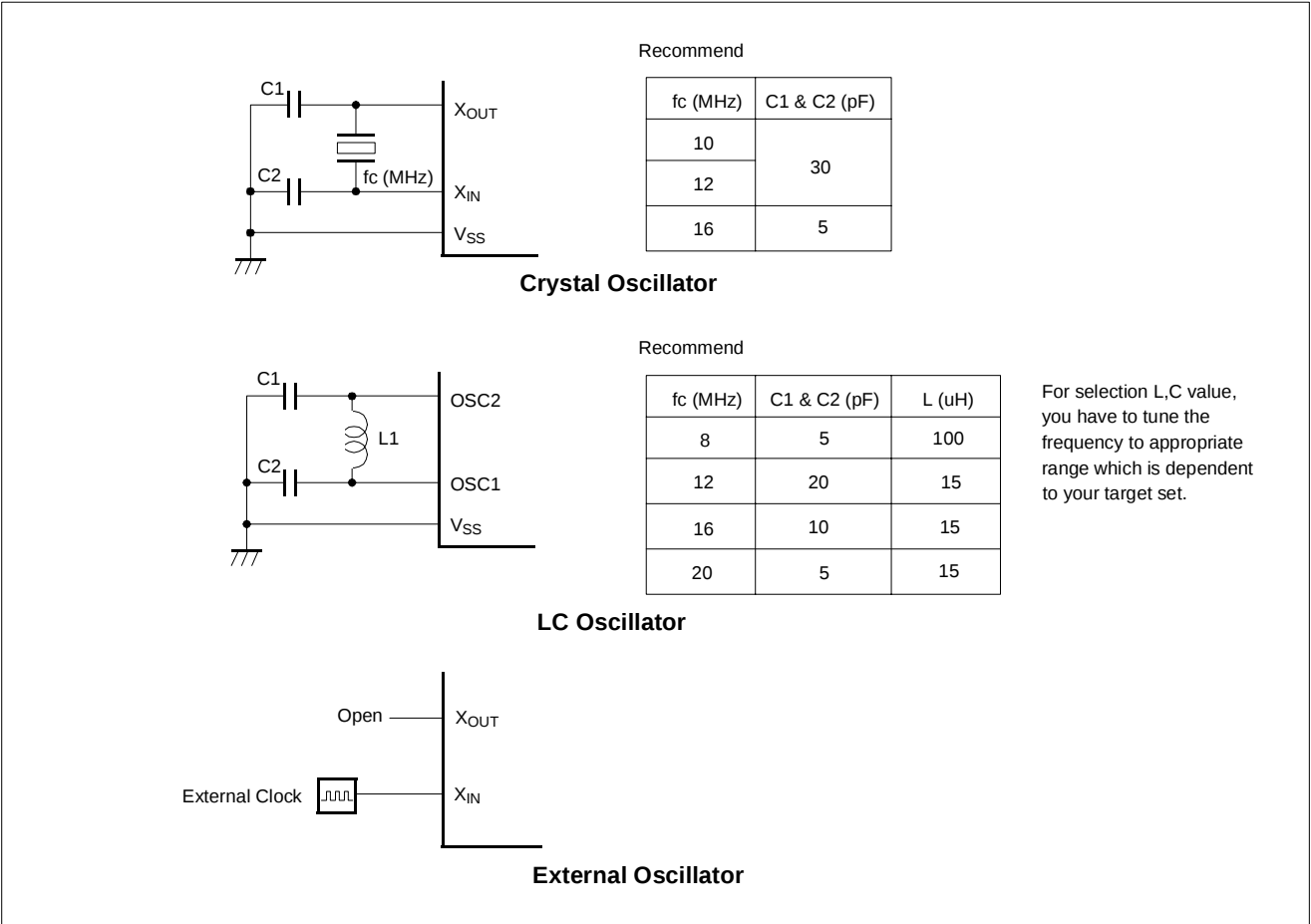
Figure 21-1 Oscillation Circuit
