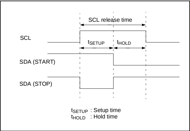
Figure 18-10 START / STOP condition detection timing
