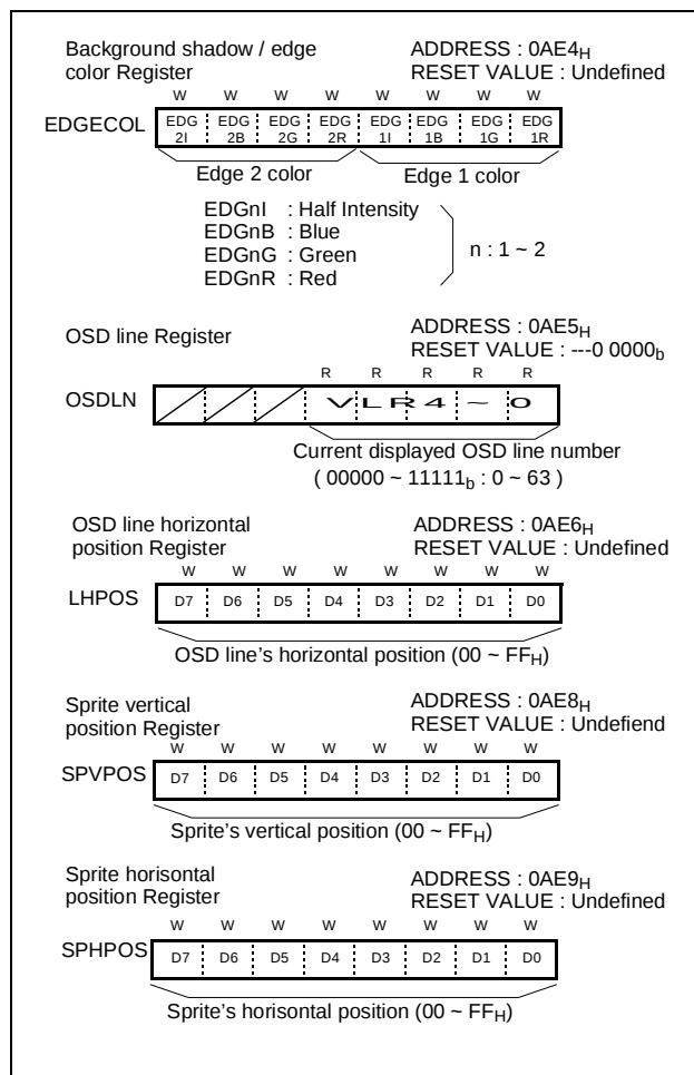
Figure 17-6 OSD Registers - 3
