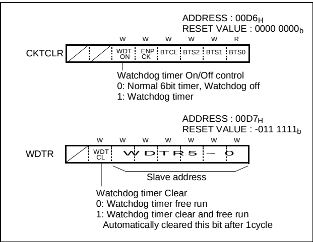
Figure 20-2 Watchdog timer register
