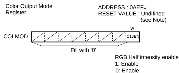
Figure 17-10 OSD Register - 7
