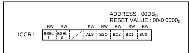
Figure 18-5 I 2 C control Register 1
