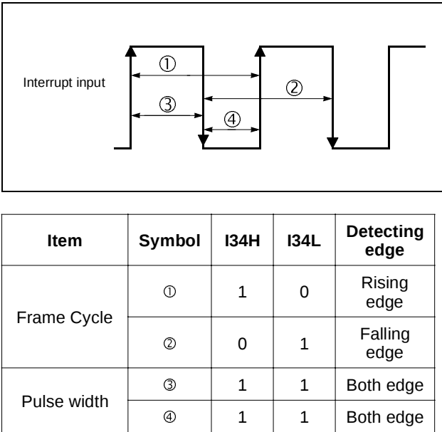
Figure 15-3 Setting for measurement
