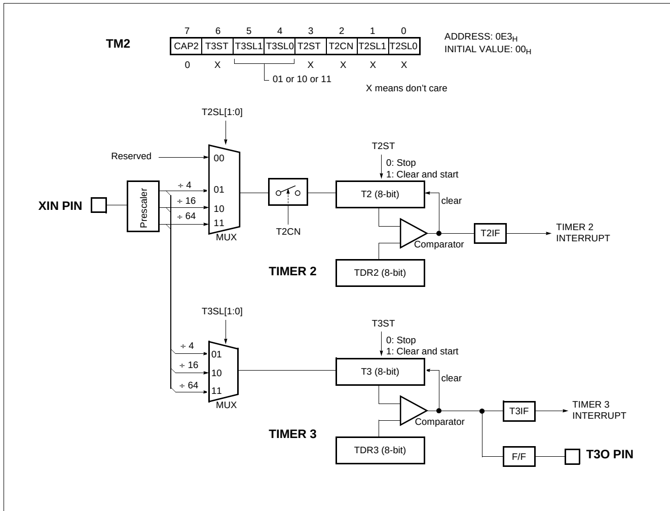
Figure 11-3 8-bit Timer/Counter 2, 3
