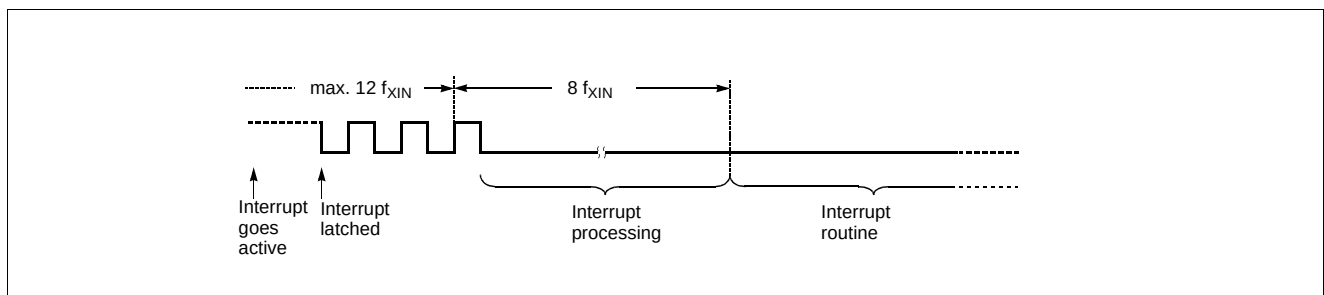
Figure 14-8 Interrupt Response Timing Diagram
