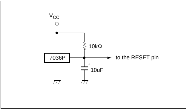
Figure 18-1 Simple Power-on-Reset Circuit
