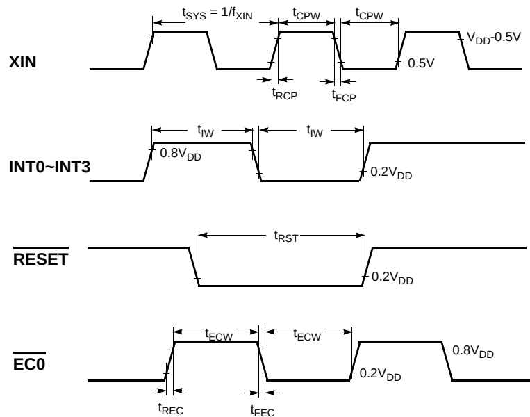
Figure 7-1 Timing Chart
