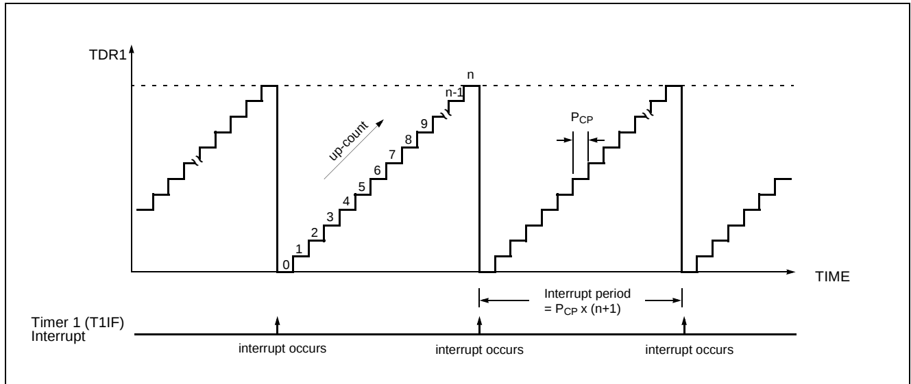
Figure 16-3 Counting Example of Timer Data Registers
