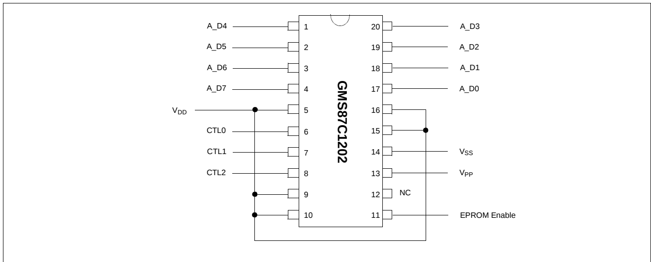
Figure 24-3 Pin Assignment
