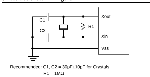
Figure 14-2 Oscillator Connections
