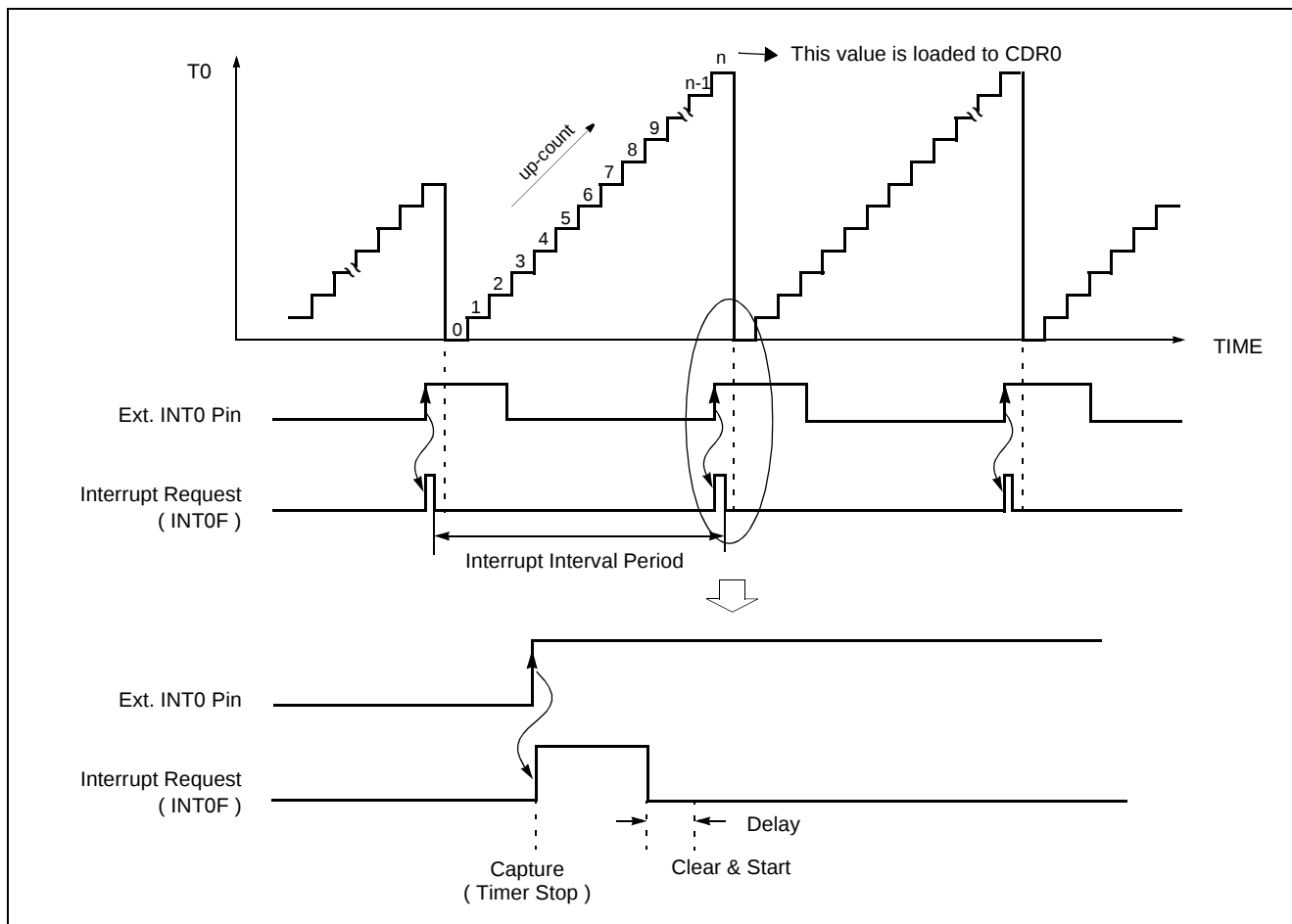
Figure 16-7 Input Capture Operation
