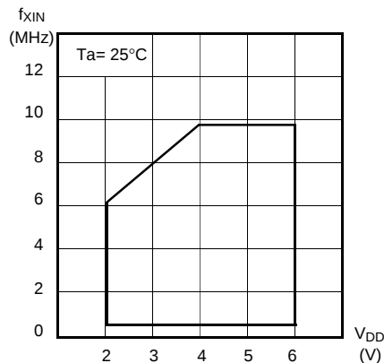
Operating Area
