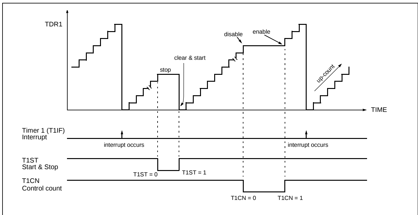
Figure 16-4 Timer Count Operation
