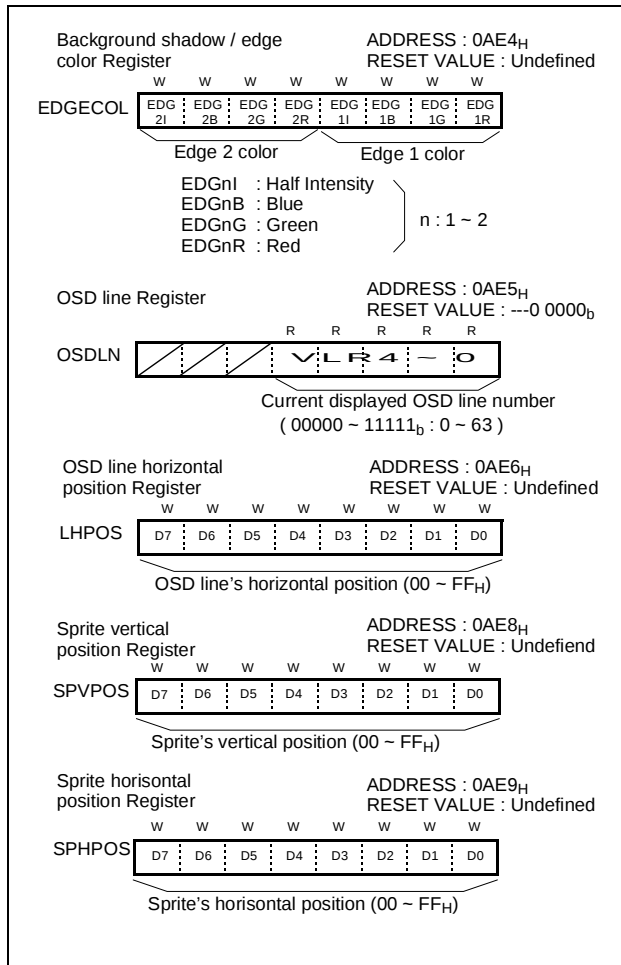
Figure 17-6 OSD Registers - 3
