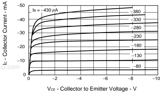
COLLECTOR CURRENT vs. COLLECTOR TO EMITTER VOLTAGE
