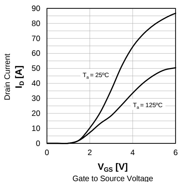
Fig.8 Typ. Transfer Characteristics
