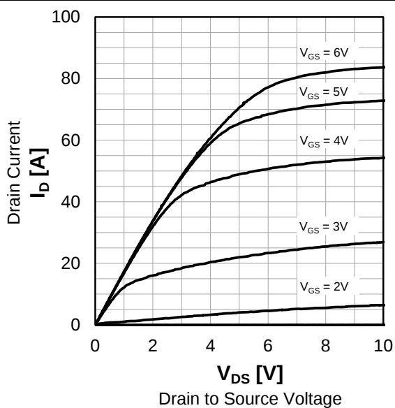
Fig.5 Typ. Output Characteristics
