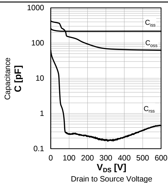
Fig.15 Typ. Capacitance
