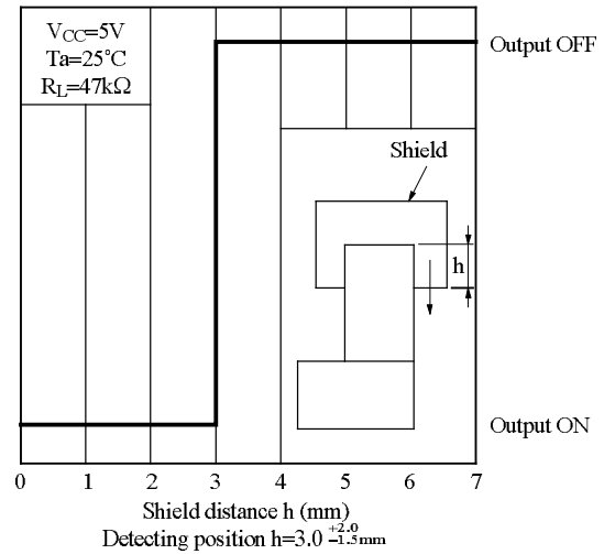
Fig.7 Detecting Position Characteristics (2)
