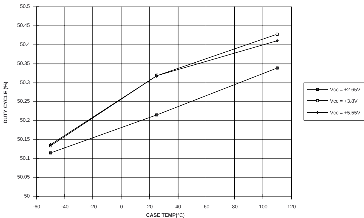
Fig. 26 Duty-cycle of SIGN digital output (pin 13), sampled at 5.71MHz in a typical application circuit - RF I/P signal = 1575.42MHz CW, -85dBm - equivalent to 26dB excess noise from a typical GPS antenna
