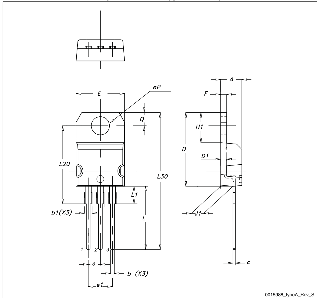
Figure 32. TO-220 type A drawing
