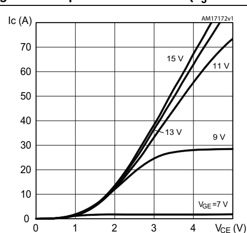
Figure 5. Output characteristics ( T_J = 175^\circ\text{C} )
