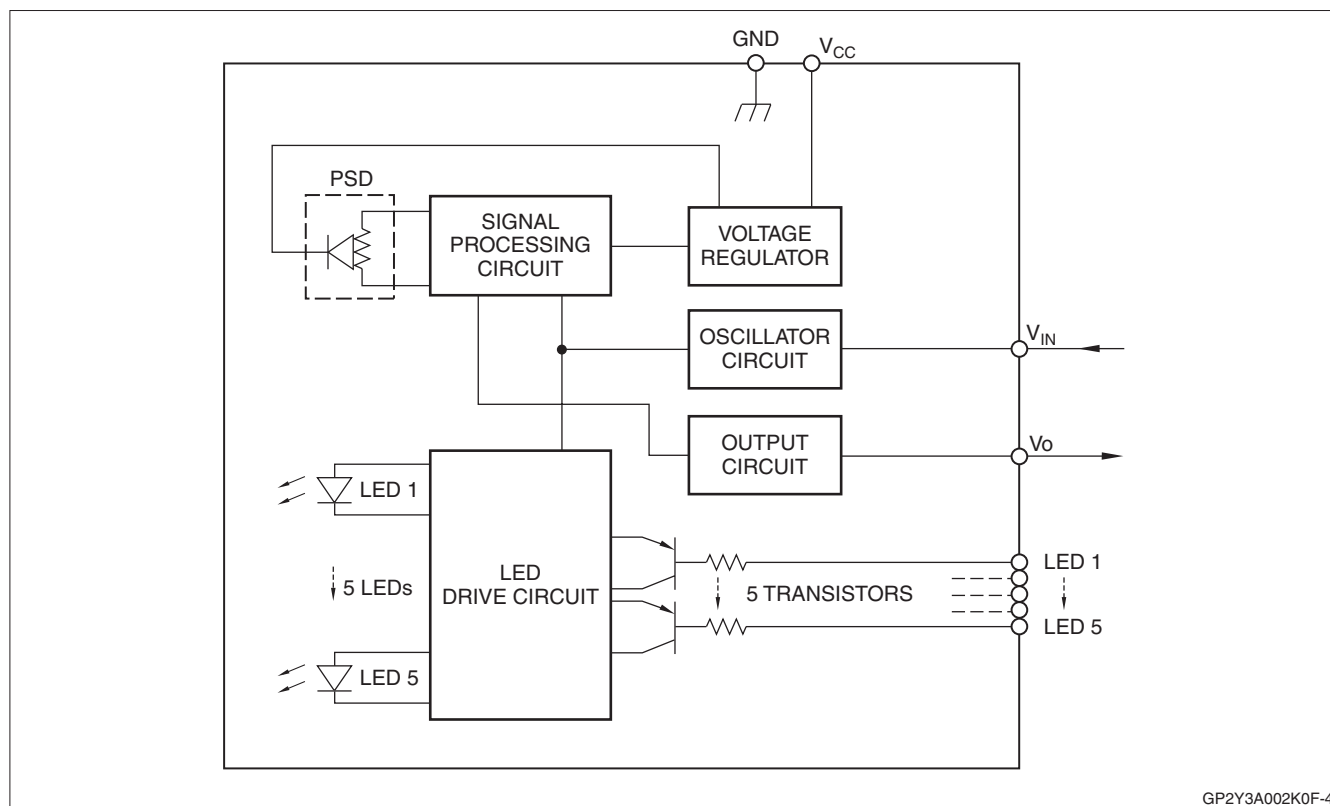
Figure 2. Block Diagram
