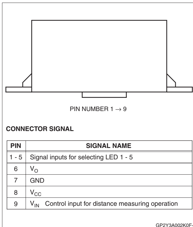
Figure 1. Pinout
