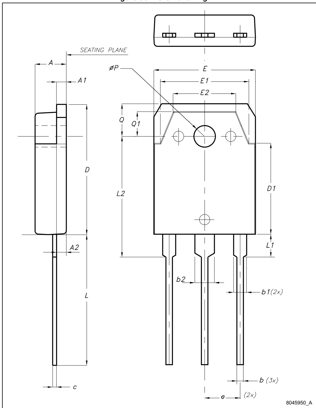
Figure 36. TO-3P drawing
