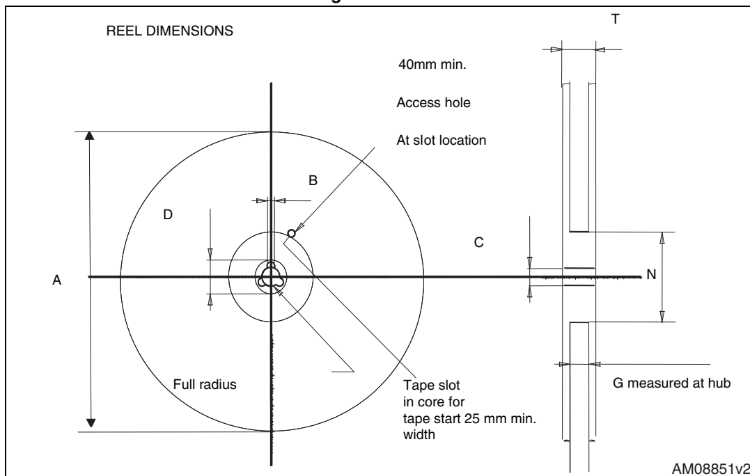
Figure 38. Reel
