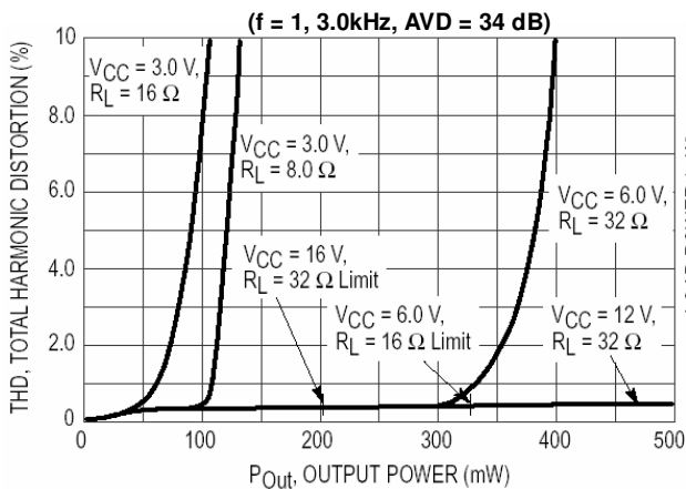
Fig 13. Distortion versus Power
